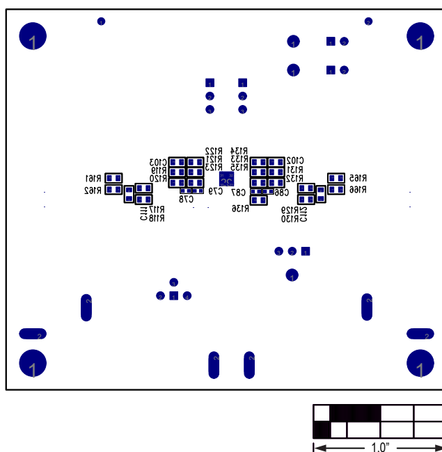
Figure 7. MAX16932 EV Kit Component Placement Guide—Solder Side
