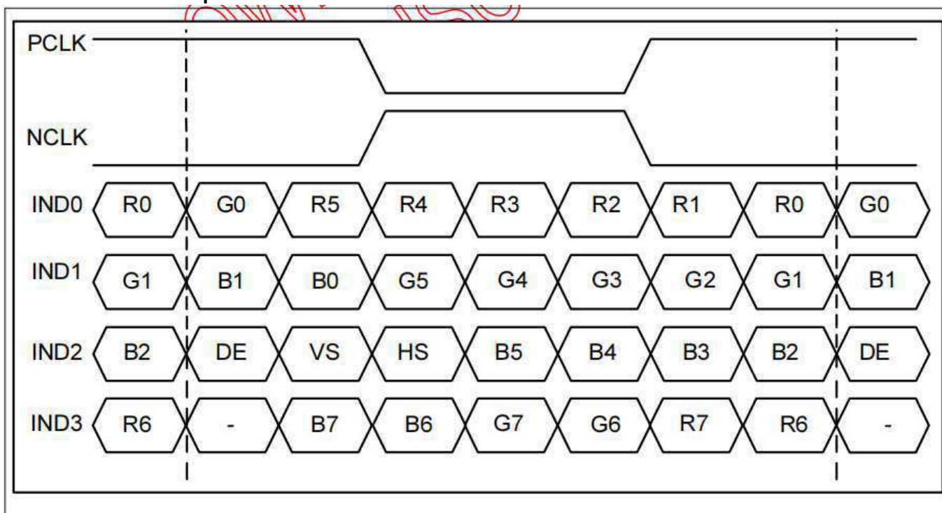
Figure 8.2 8 bit Lvds data input
