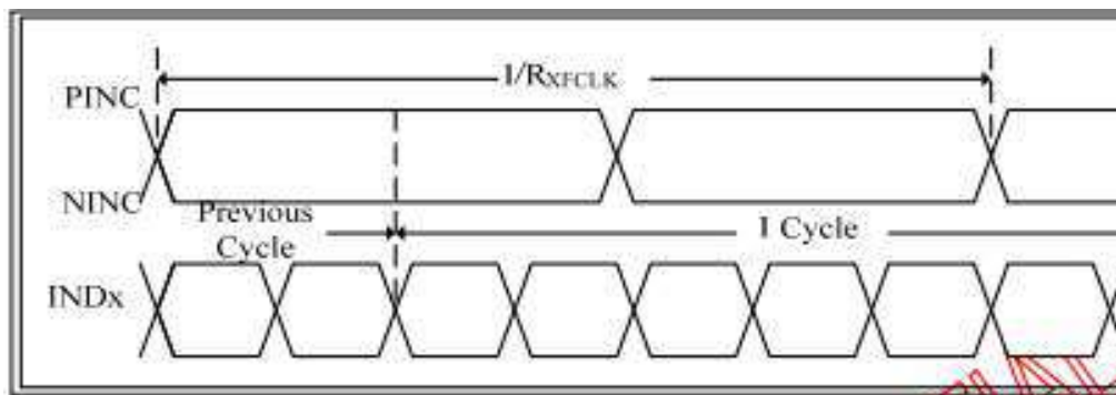
LVDS timing(1)
