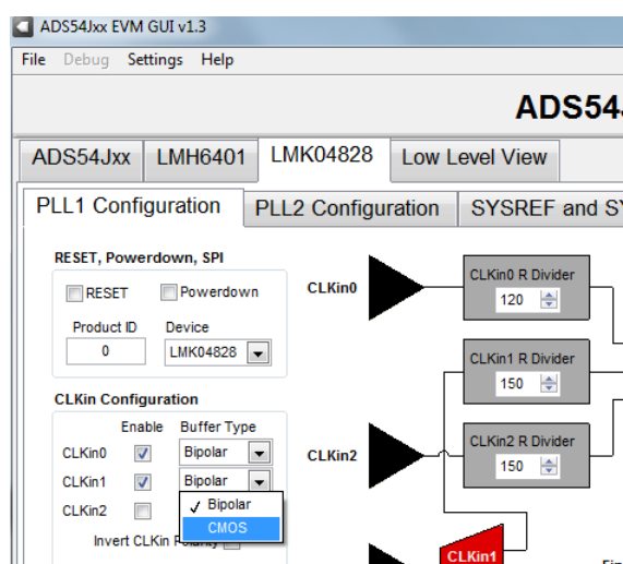
Figure 8. GUI CMOS Selection
