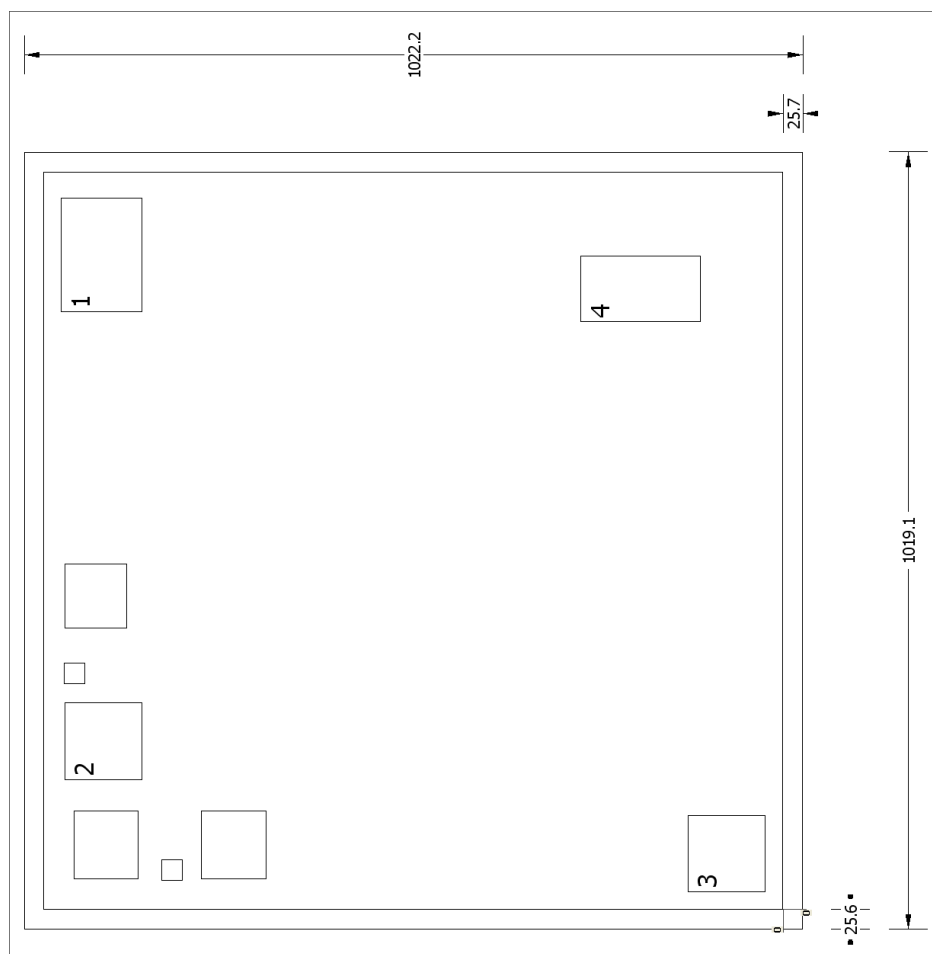
Bond Pad Coordinates in Microns
