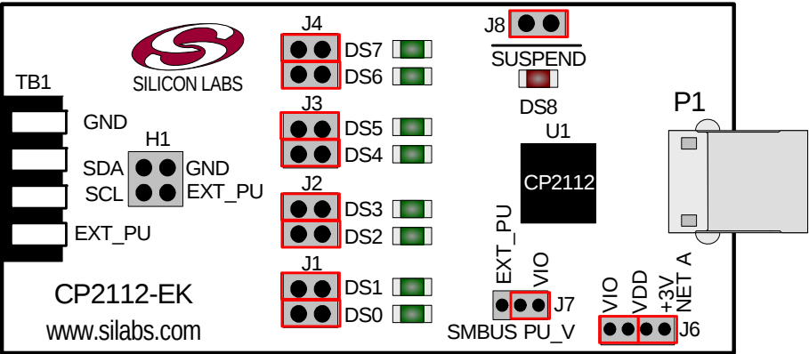
Figure 9. CP2112 Evaluation Board with Default Shorting Blocks Installed
