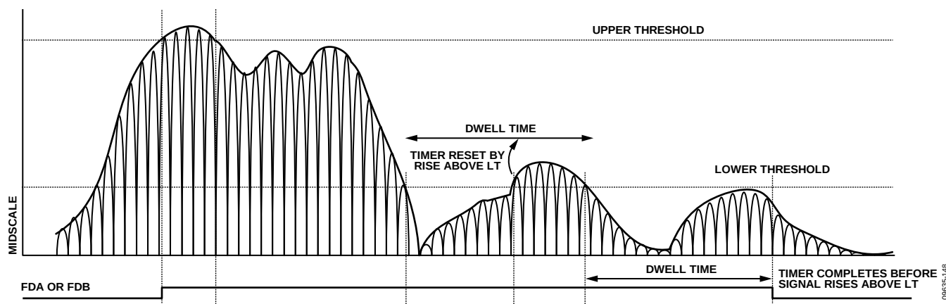
Figure 45. Threshold Settings for FDA and FDB Signals
