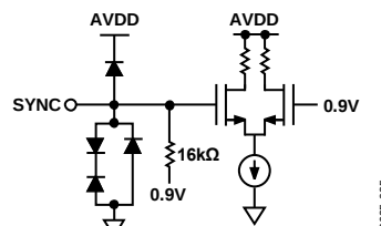
Figure 25. Equivalent SYNC Input Circuit
