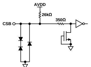
Figure 24. Equivalent CSB Input Circuit
