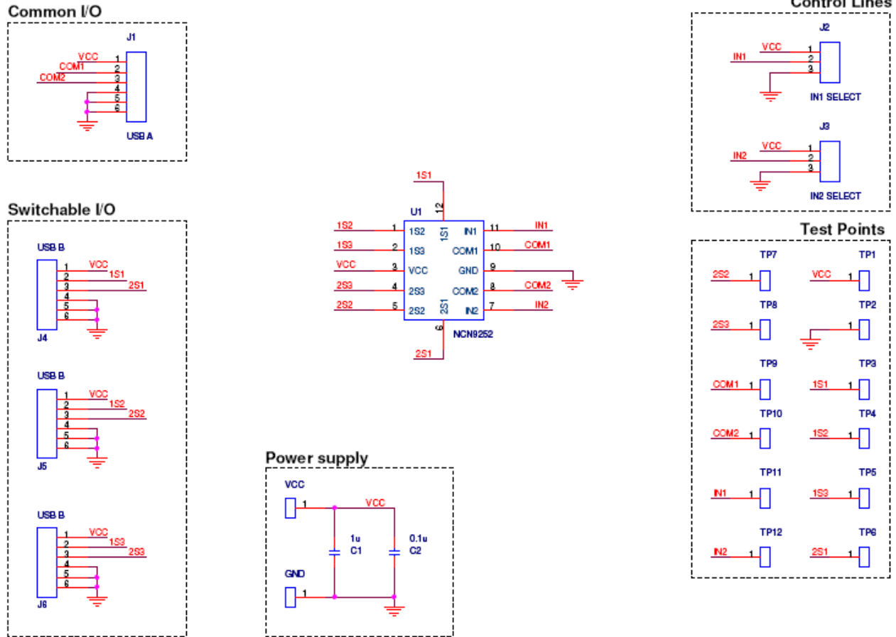
Figure 3. Board Schematic
