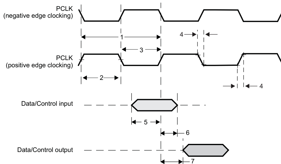
Figure 8-46. ISSCAM Timings
