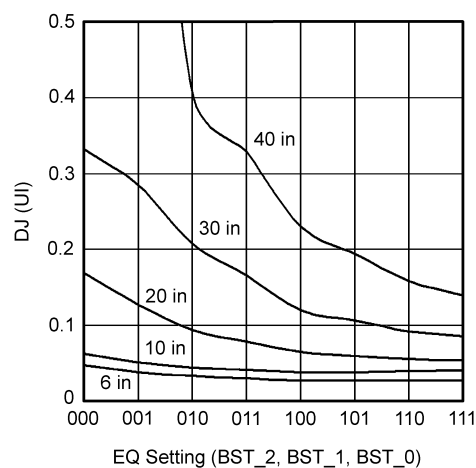
Figure 12. DJ vs. EQ Setting (3.2 Gbps)
