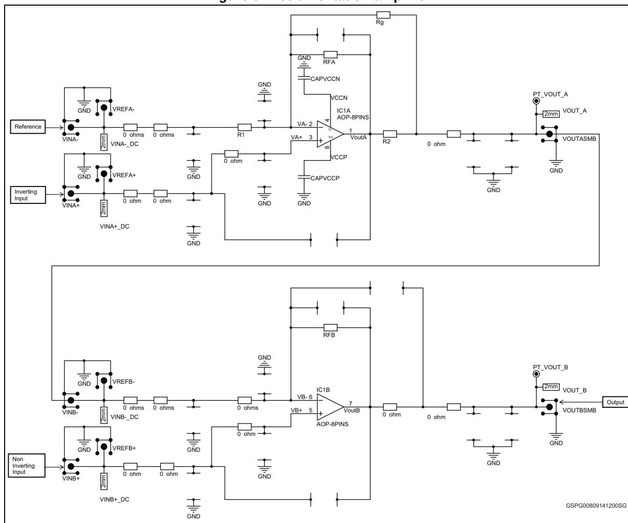
Figure 8. Instrumentation amplifier
