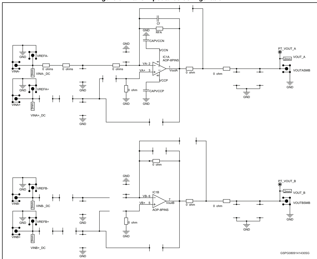
Figure 9. Transimpedance configuration
