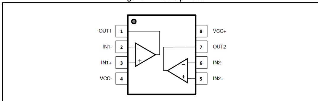
Figure 1. MSO8 pinout
