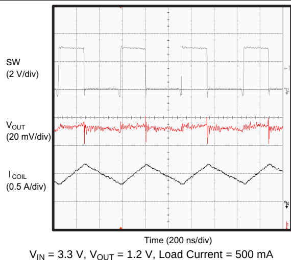
Figure 23. Typical Application (PWM Mode)
