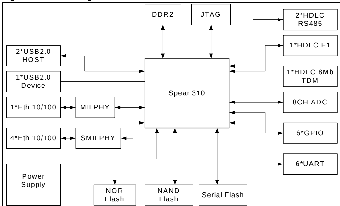
Figure 3. Block diagram
