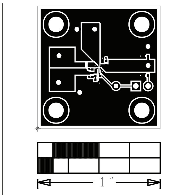
MAX40000 EV Kit—Top
