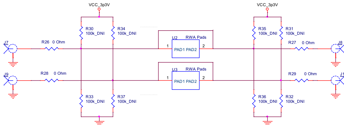
Figure 3. HD3SS3411 EVM Schematic Cal Trace
