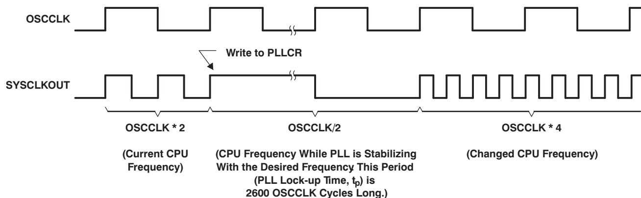
Figure 5-5. Example of Effect of Writing Into PLLCR Register
