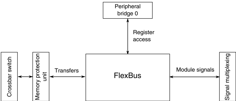
Figure 3-30. FlexBus configuration
