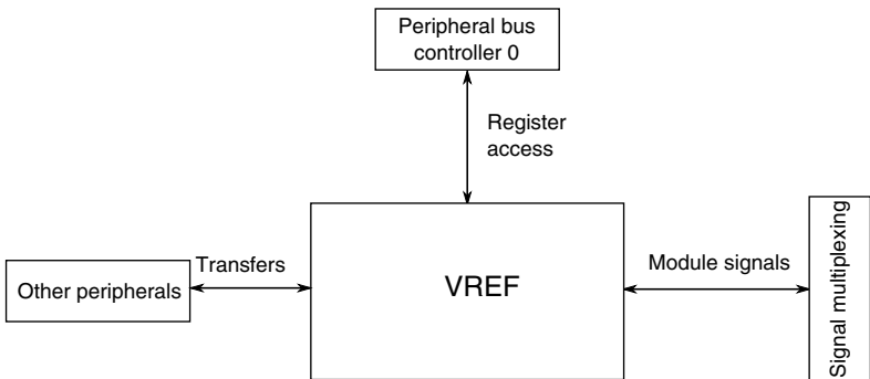
Figure 3-39. VREF configuration
