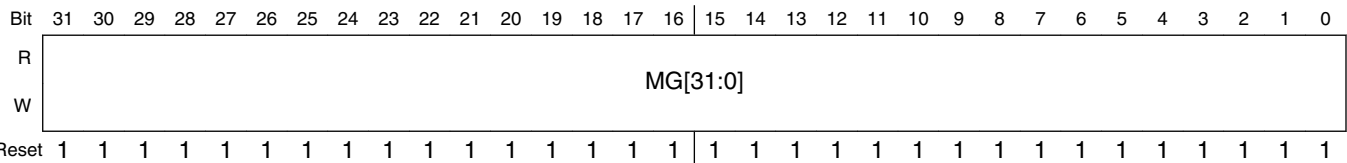
CANx_RXMGMASK field descriptions
