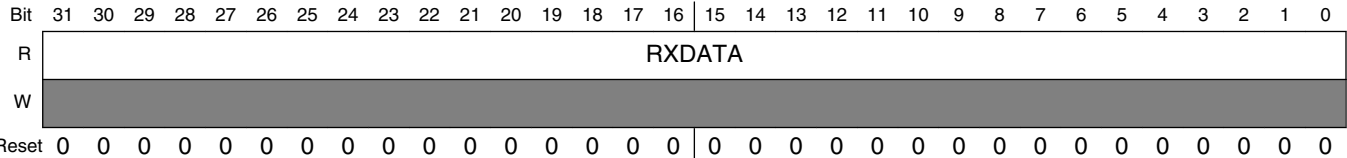
SPIx_RXFRn field descriptions
