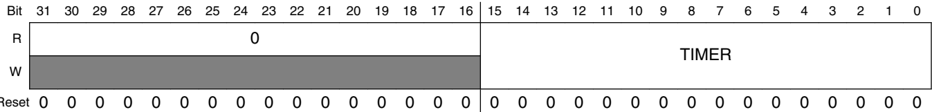
CANx_TIMER field descriptions
