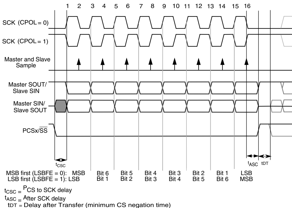
Figure 46-73. DSPI Transfer Timing Diagram (MTFE=0, CPHA=1, FMSZ=8)
