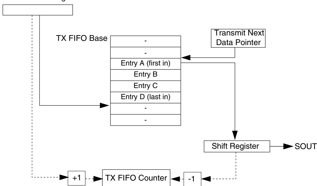
Figure 46-78. TX FIFO Pointers and Counter
