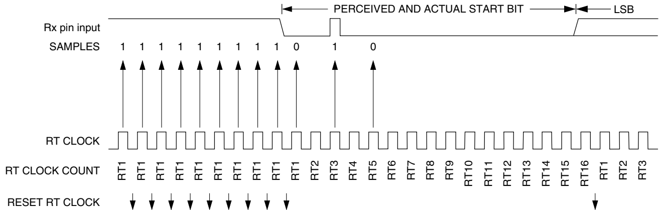
Figure 48-163. Start bit search example 4 (C7816[ISO_7816E] = 0)
