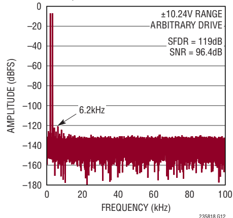
32k Point Arbitrary Two-Tone FFT f_{SAMPL} = 200\text{kHz} , IN^+ = -7\text{dBFS } 2\text{kHz} Sine, IN^- = -7\text{dBFS } 3.1\text{kHz} Sine
