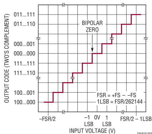
Figure 2. LTC2358-18 Two's Complement Transfer Function
