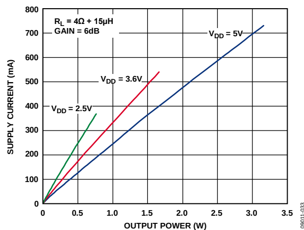
Figure 30. Supply Current vs. Output Power into 4Ω, Gain = 6 dB
