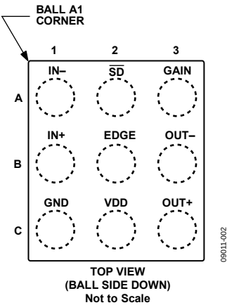
Figure 2. Pin Configuration
