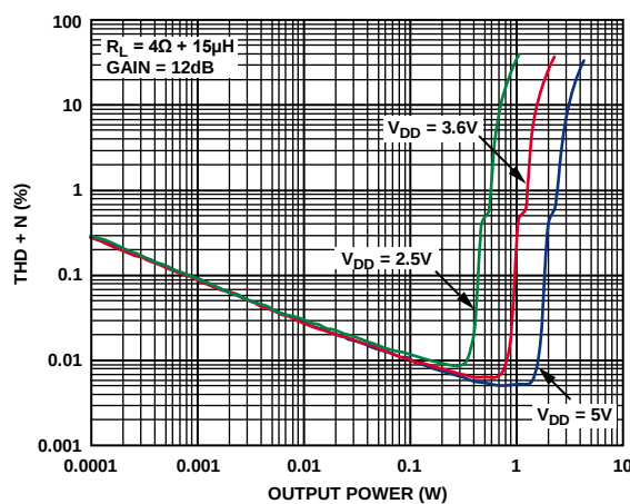
Figure 7. THD + N vs. Output Power into 4 Ω, Gain = 12 dB
