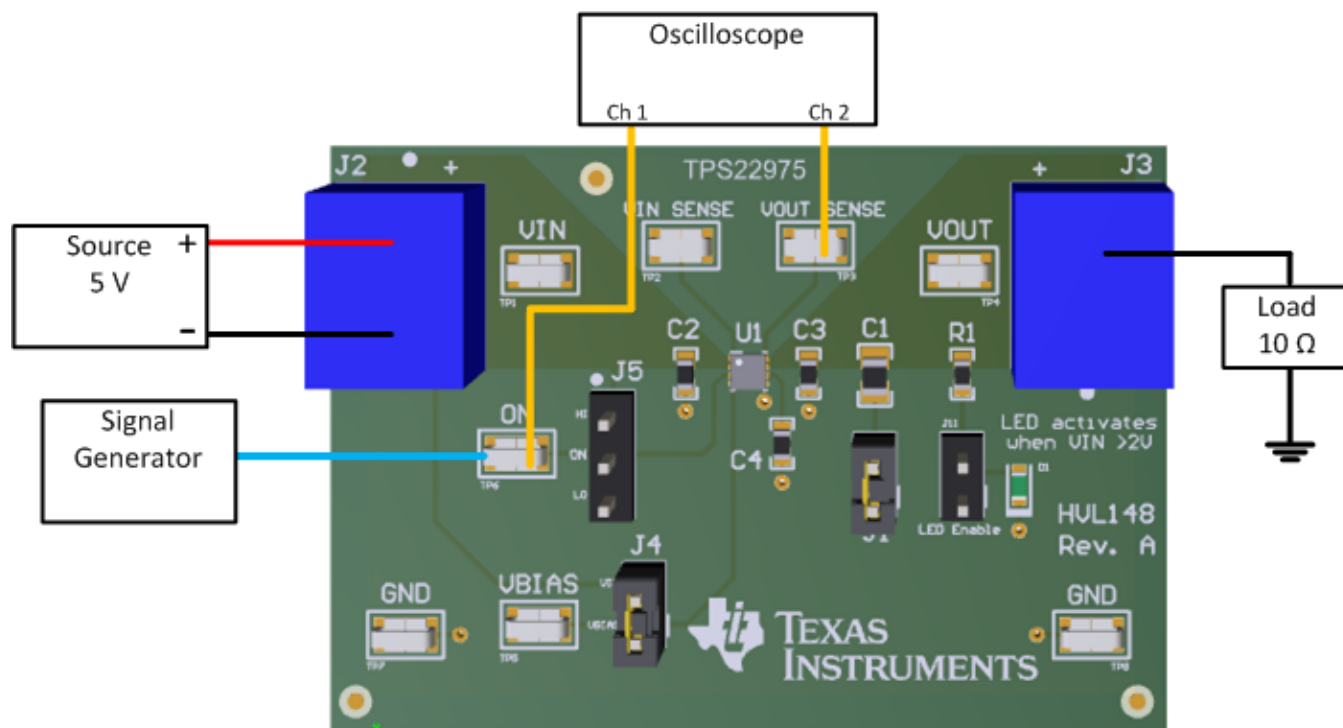
Figure 5. Rise Time Test Setup
