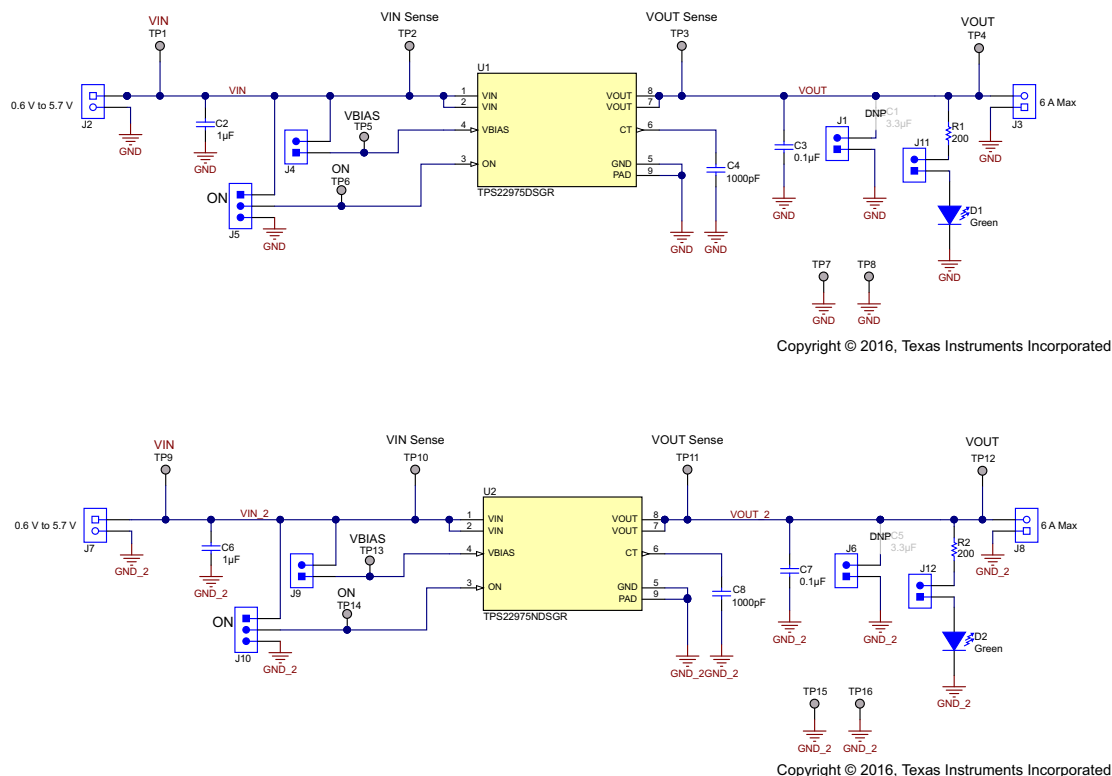
Figure 1. TPS22975EVM Schematic
