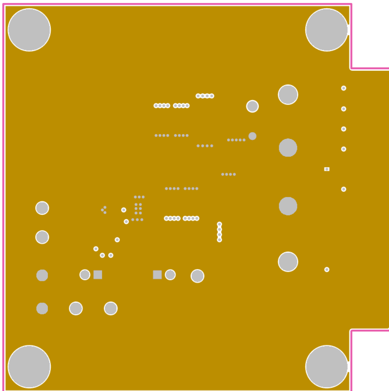
Figure 3. Middle Layer 1
