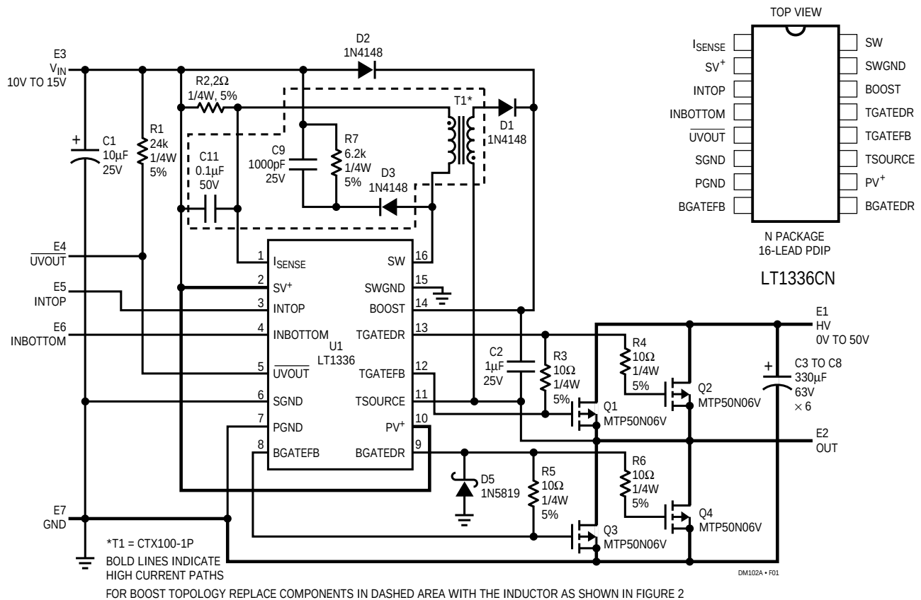
Figure 1. Demonstration Circuit with a Flyback High-Side Driver Regulator
