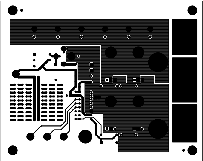
Component Side
