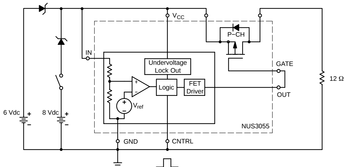
Figure 11. Test Circuit for T_{\text{ON CT}} and T_{\text{OFF CT}}
