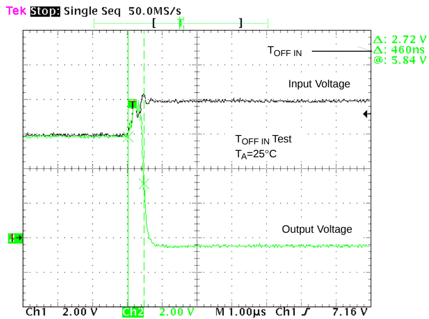
Figure 10. T_{\text{OFF IN}} Waveforms
