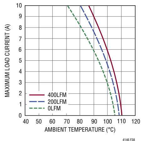
Figure 38. 36V IN to 1.5V OUT No Heat Sink, f_{SW} = 315\text{kHz} at Full Load
