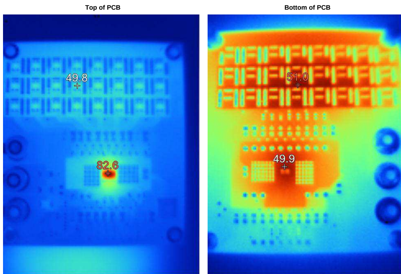
Figure 4. Thermal Performance of Low Current
