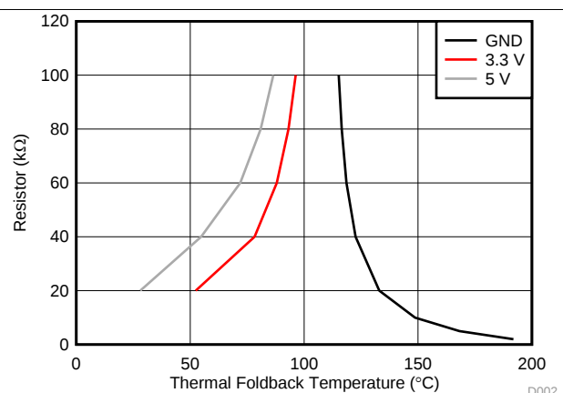
Figure 8. Pullup and Pulldown Resistors vs T_{\text{th}}
