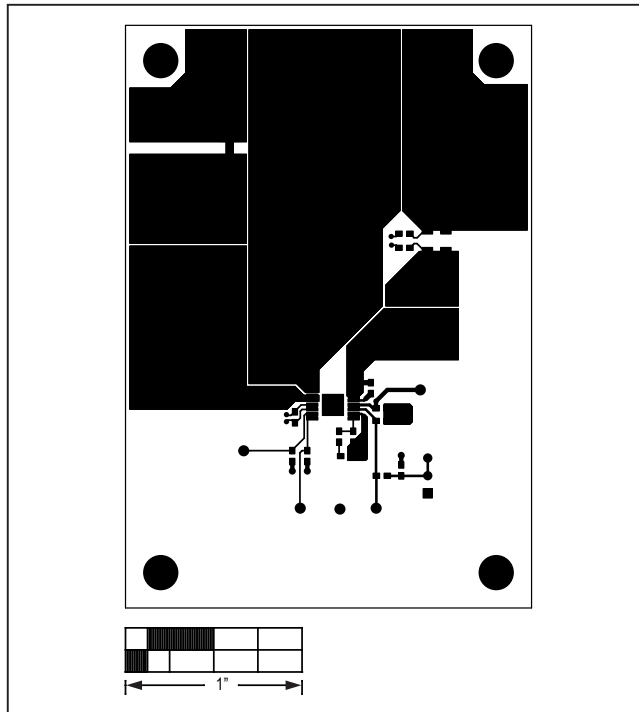
Figure 3. MAX20051 EV Kit PCB Layout—Component Side
