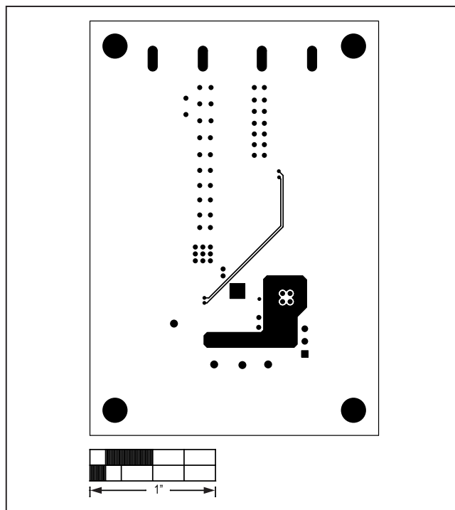
Figure 5. MAX20051 EV Kit PCB Layout—VCC Layer 3
