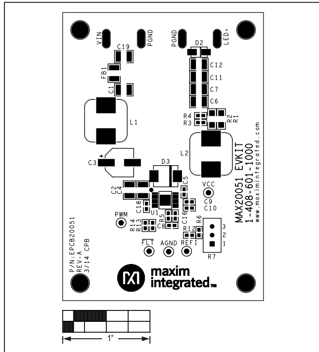
Figure 2. MAX20051 EV kit Component Placement Guide—Component Side
