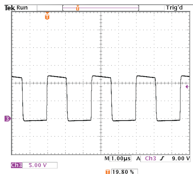
Figure 3. PH Node at 1-A Load
