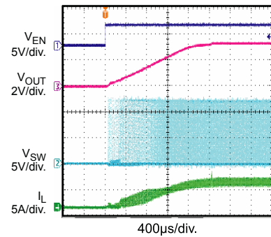
Enable Startup With 6A Load (Resistive)
