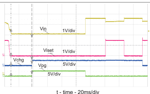
Figure 30. DPM – USB Current Limits – Vin Regulated to 4.4V
