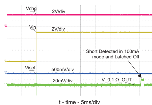
Figure 28. ISET Shorted Prior to USB Power-up
