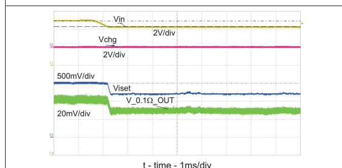
Figure 27. ISET Shorted During Normal Operation
