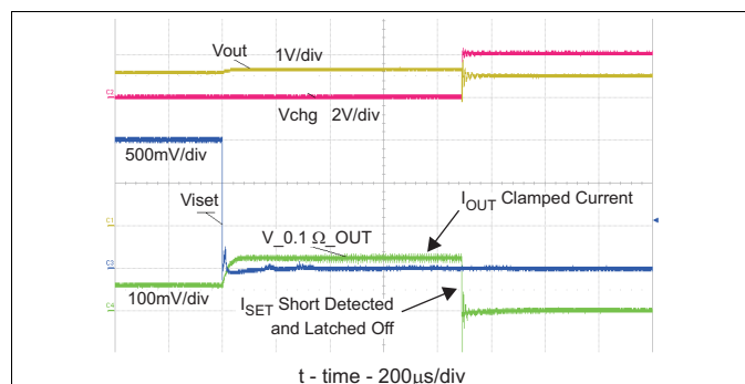
Figure 27. ISET Shorted During Normal Operation
