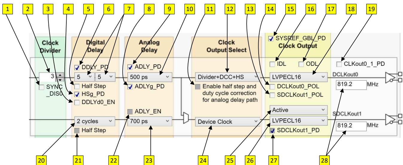
Figure 2. CLKout Page Description Diagram
