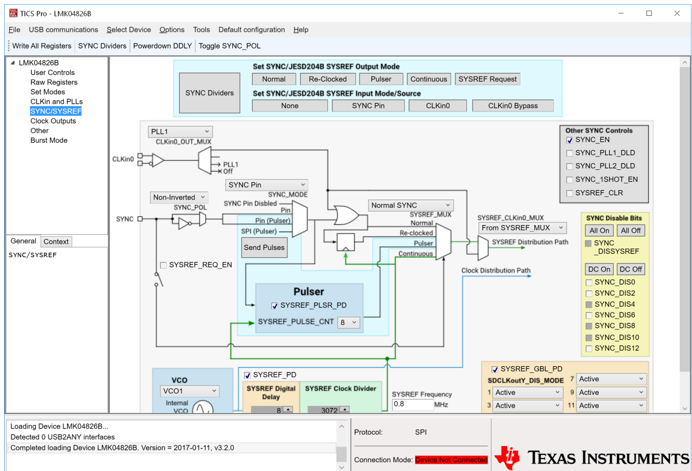
Figure 15. TICS Pro - SYNC / SYSREF Page
