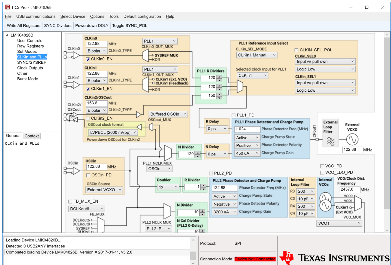
Figure 14. TICS Pro - CLKinX Control Page
