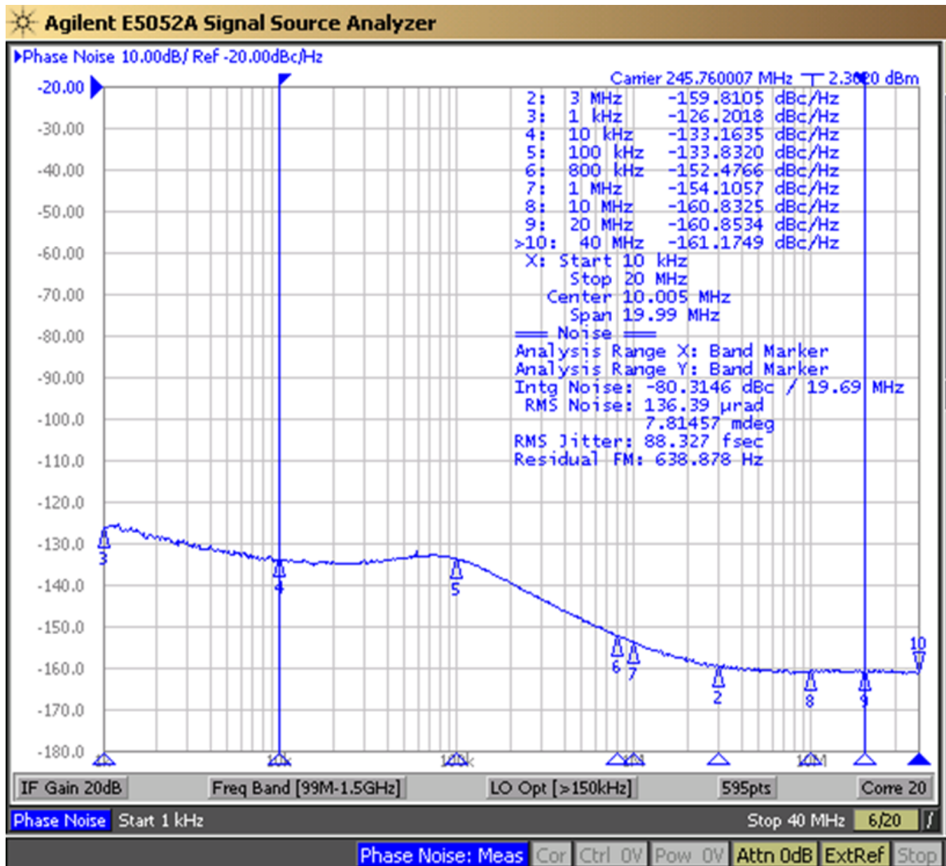
Figure 23. LMK04826 DCLKout2, VCO1, 245.76 MHz, Div10 , LVPECL20 /w 240- \Omega Emitter Resistor, DCLKoutX_MUX=Divider, IDL=1, ODL=0, Single Ended
