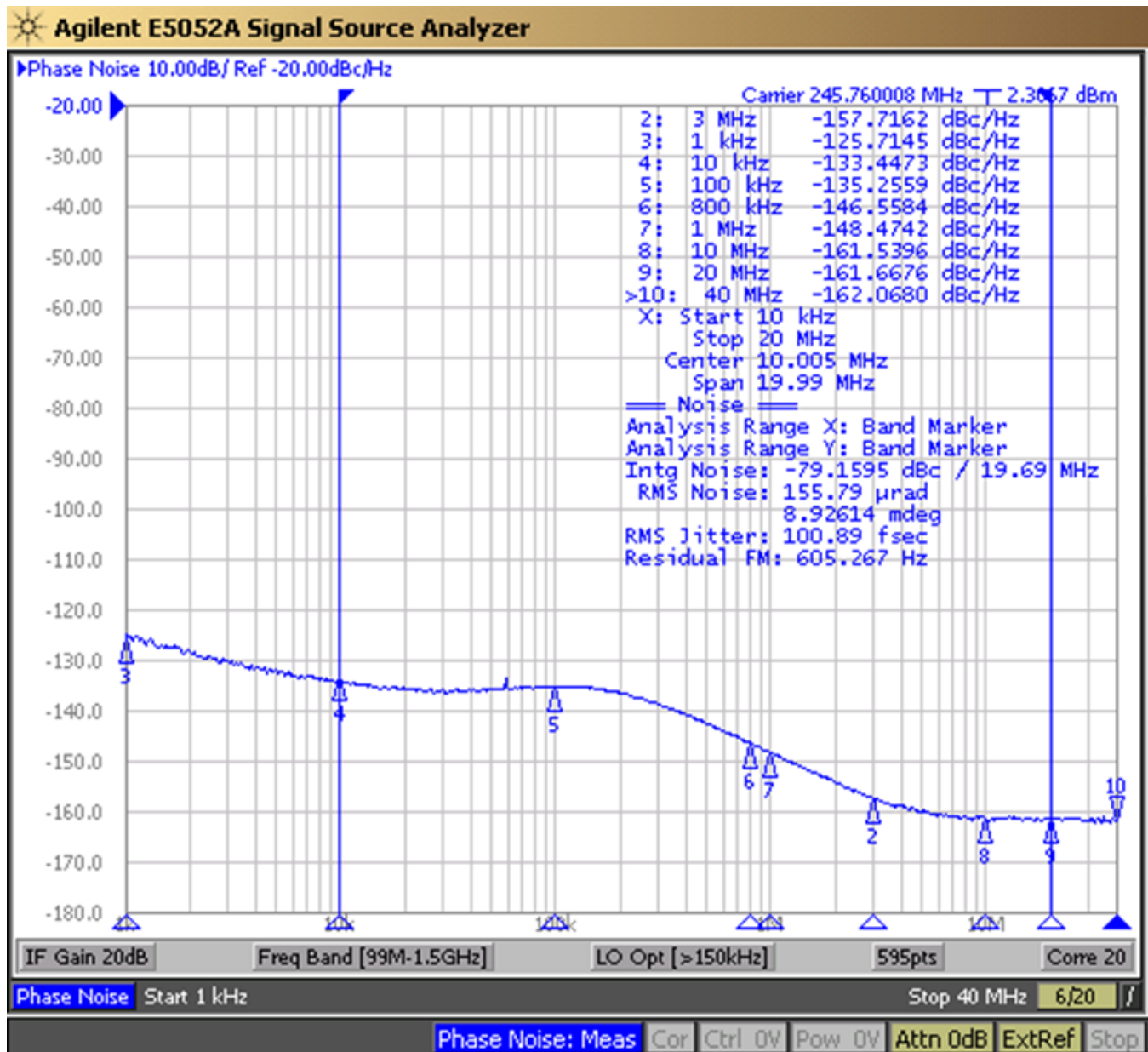
Figure 21. LMK04826 DCLKout2, VCO0, 245.76 MHz, Div8, LVPECL20 /w 240- \Omega Emitter Resistor, DCLKoutX_MUX=Divider, IDL=1, ODL=0, Single Ended
