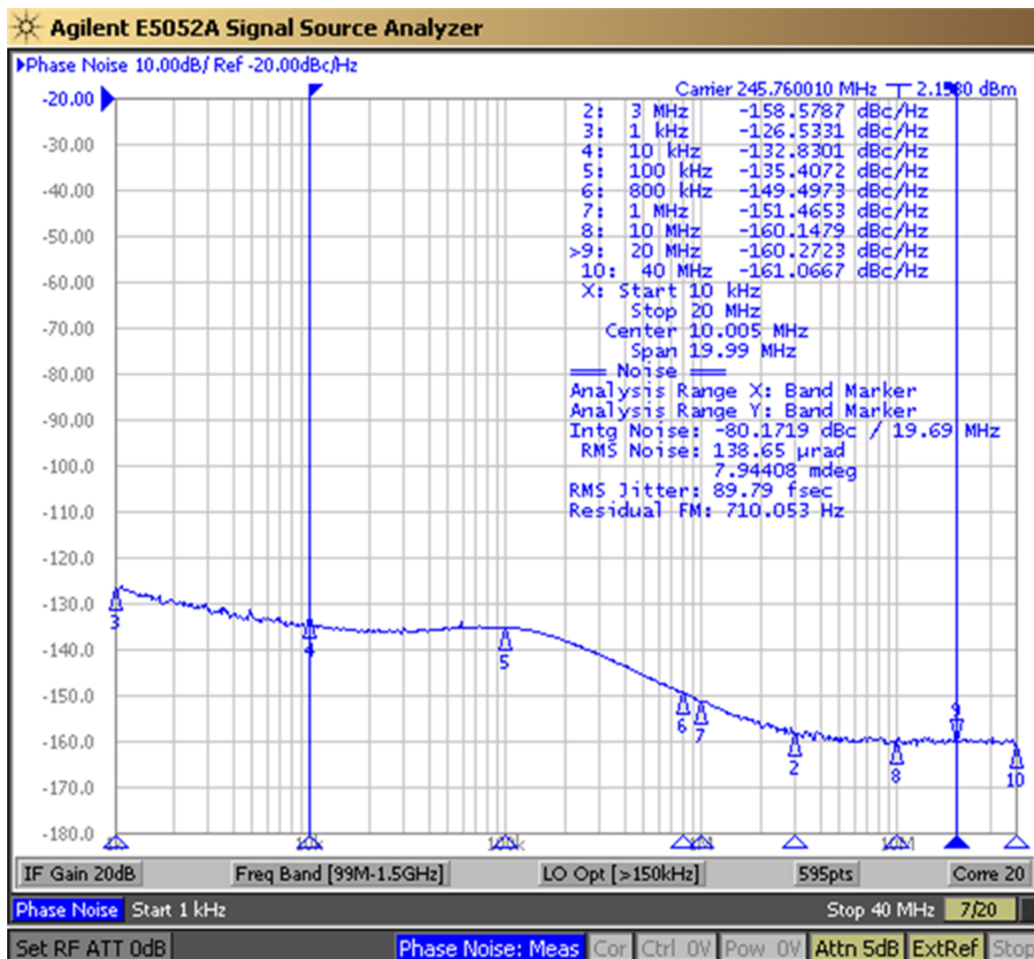
Figure 27. LMK04828 DCLKout2, VCO1, 245.76 MHz, Div12, LVPECL20 /w 240- \Omega Emitter Resistor, DCLKoutX_MUX=Divider, IDL=1, ODL=0, Single Ended
