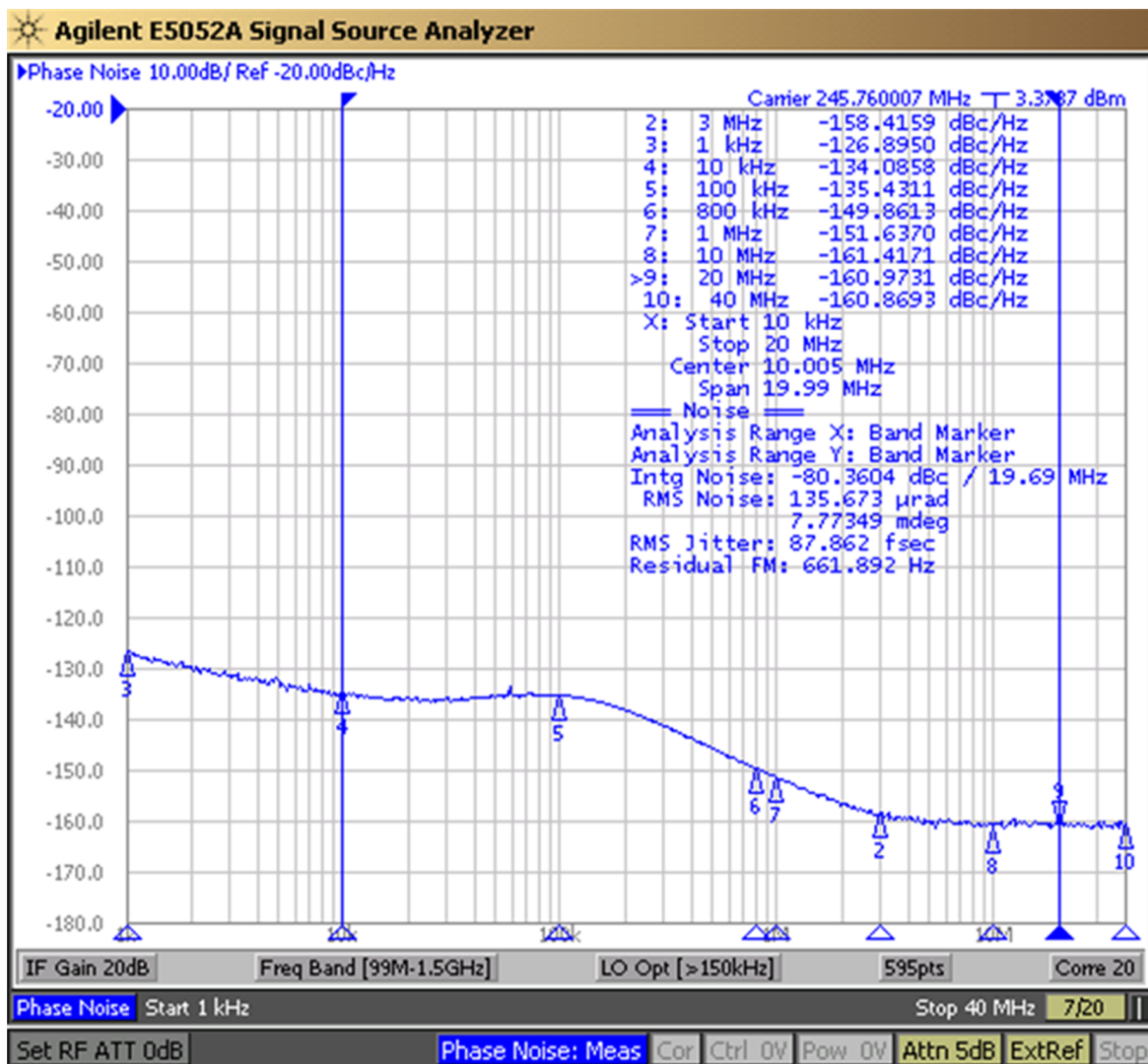
Figure 26. LMK04828 DCLKout2, VCO1, 245.76 MHz, Div12, LVPECL20 /w 240- \Omega Emitter Resistor, DCLKoutX_MUX=Divider, IDL=1, ODL=0, Balun = ADT2-1T
