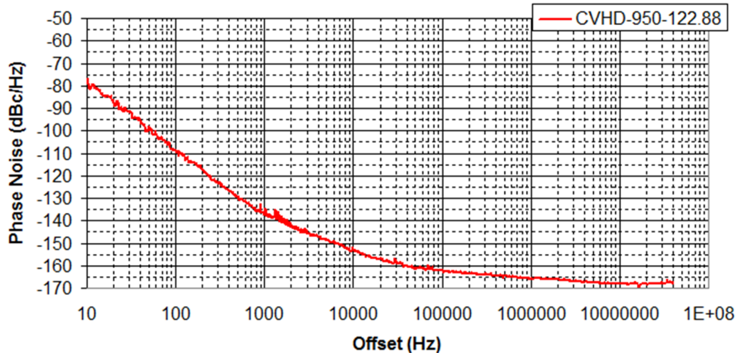
Figure 19. Crystek CVHD-950-122.88 MHz VCXO Phase Noise at 122.88 MHz
