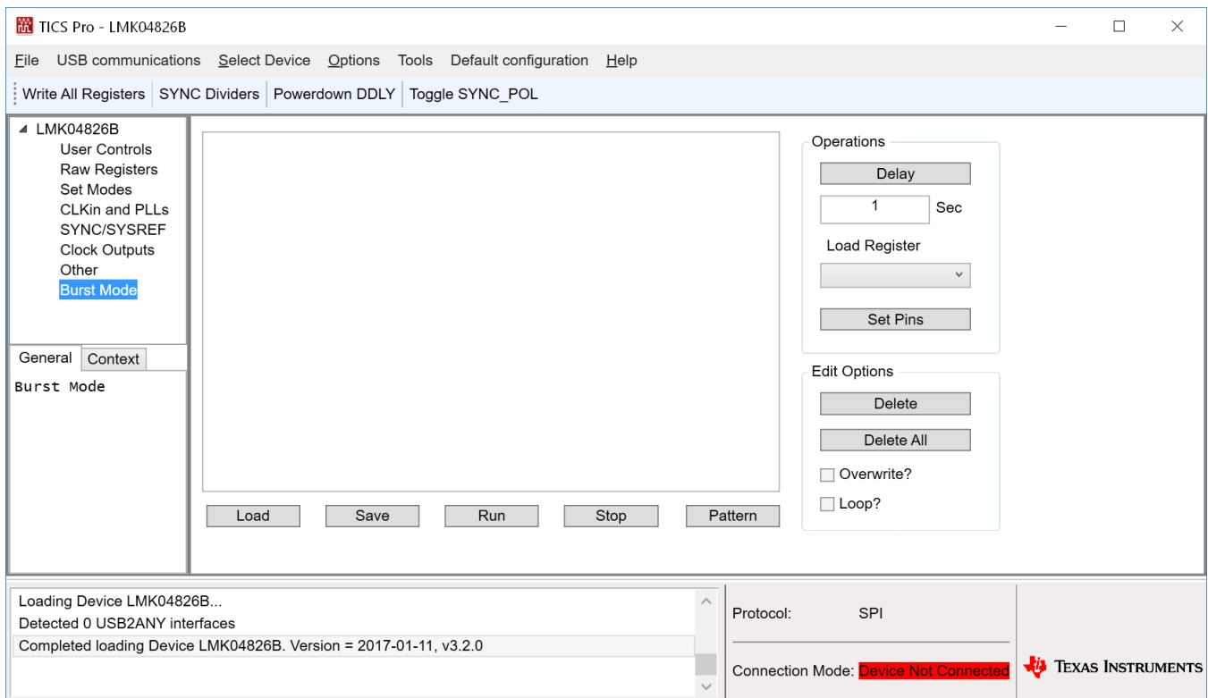
Figure 18. TICS Pro - Burst Page
