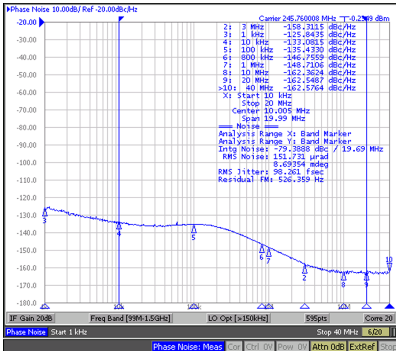
Figure 20. LMK04826 DCLKout2, VCO0, 245.76 MHz, Div8, LVPECL20 /w 240- \Omega Emitter Resistor, DCLKoutX_MUX=Divider, IDL=1, ODL=0, Balun = Prodyn BIB-100G
