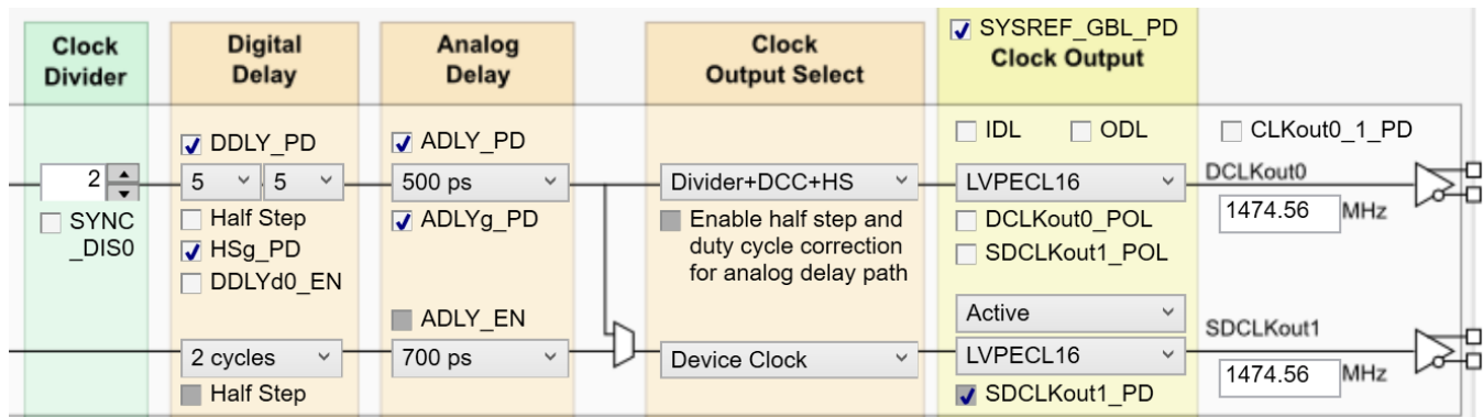
Figure 10. Setting Digital Delay, Clock Divider, Analog Delay and Output Format
