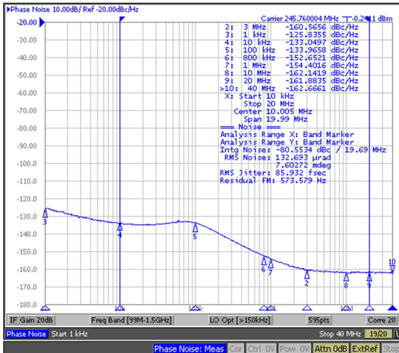
Figure 22. LMK04826 DCLKout2, VCO1, 245.76 MHz, Div10, LVPECL20 /w 240 ohm emitter resistor, DCLKoutX_MUX=Divider, IDL=1, ODL=0, Balun = Prodyn BIB-100G
