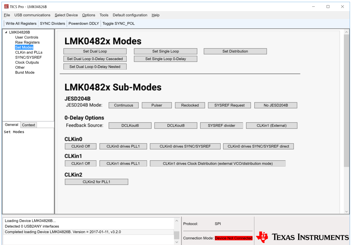
Figure 13. TICS Pro - Set Modes Page
