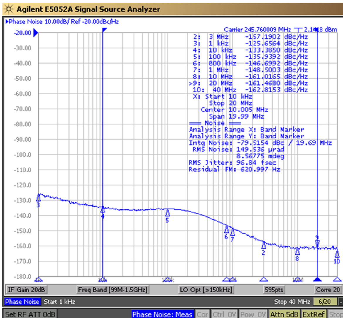
Figure 25. LMK04828 DCLKout2, VCO0, 245.76 MHz, Div10, LVPECL20 /w 240- \Omega Emitter Resistor, DCLKoutX_MUX=Divider, IDL=1, ODL=0, Single Ended
