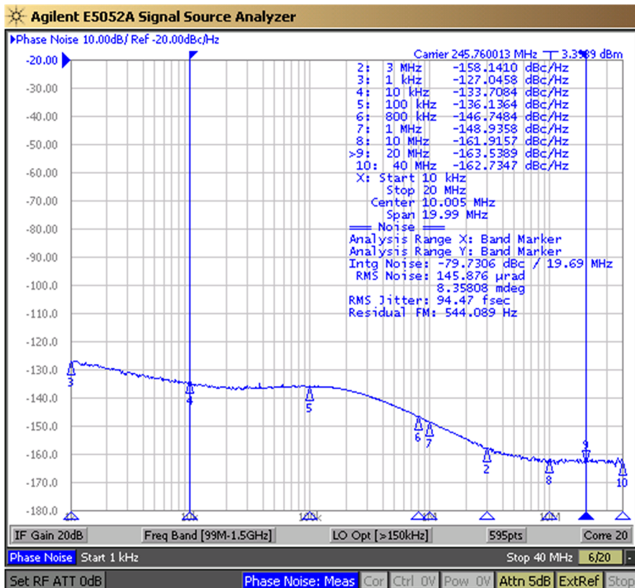
Figure 24. LMK04828 DCLKout2, VCO0, 245.76 MHz, Div10, LVPECL20 /w 240- \Omega Emitter Resistor, DCLKoutX_MUX=Divider, IDL=1, ODL=0, Balun = ADT2-1T
