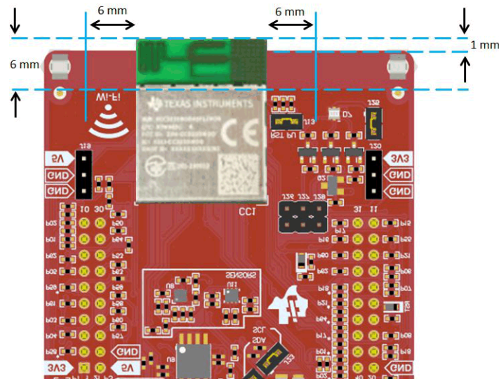
Figure 7-9. CC3235MODAx Layout Guidelines
