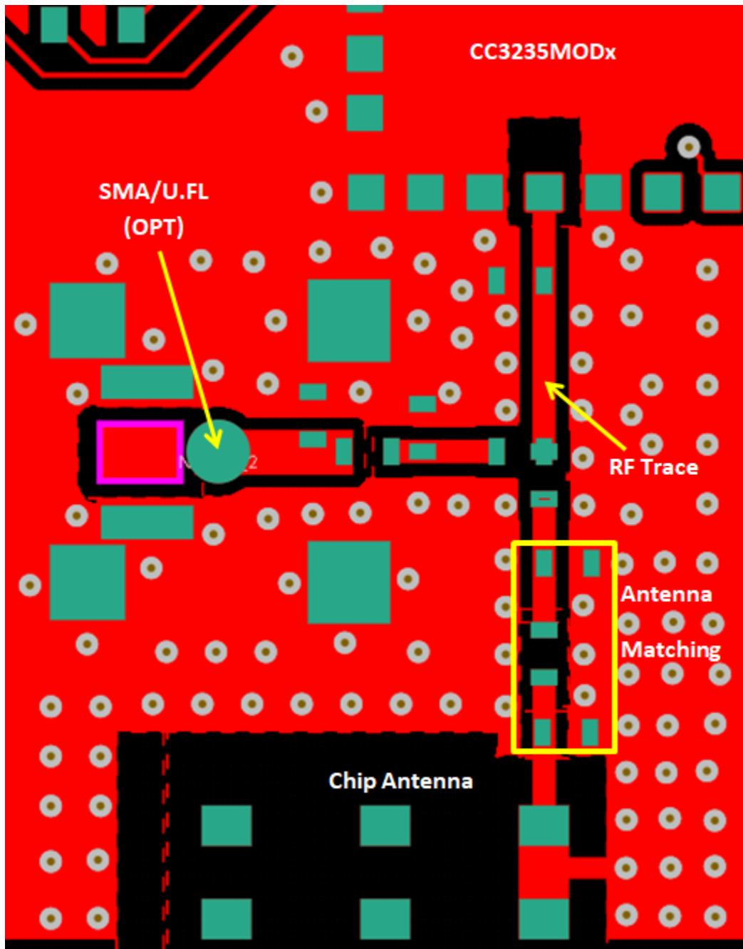
Figure 7-5. RF Section Layout
