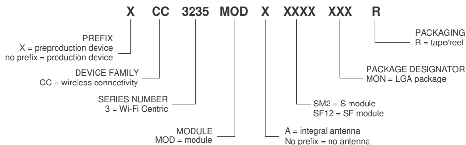
Figure 9-1. CC3235MODx and CC3235MODAx Module Nomenclature
