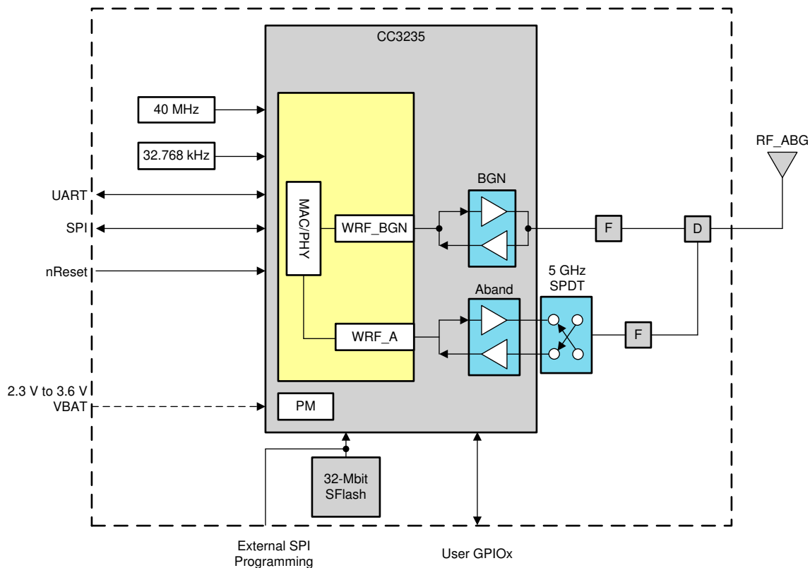
Figure 1-1. CC3235MODx Functional Block Diagram
