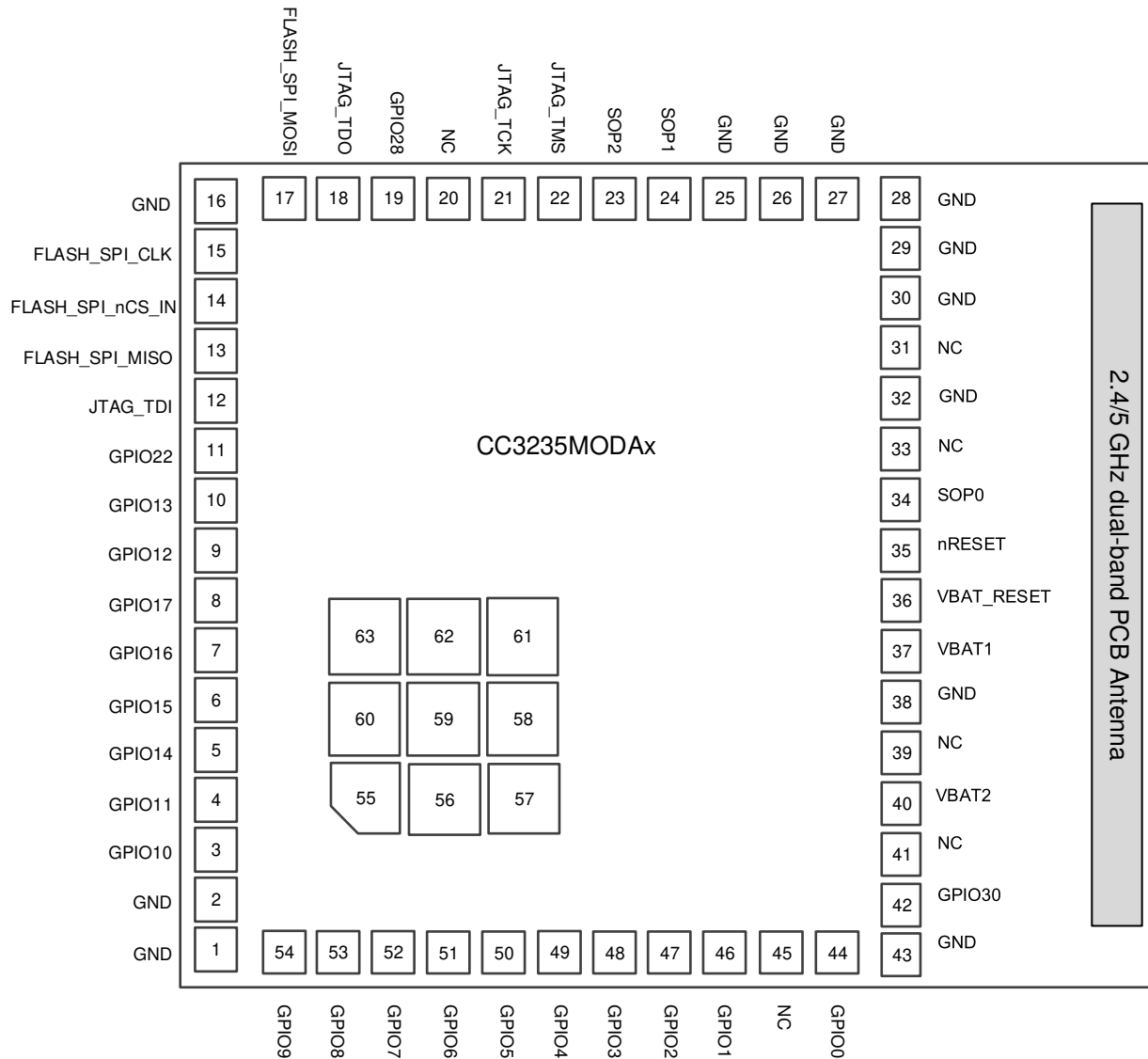
Figure 4-2. CC3235MODAx Pin Diagram Bottom View
