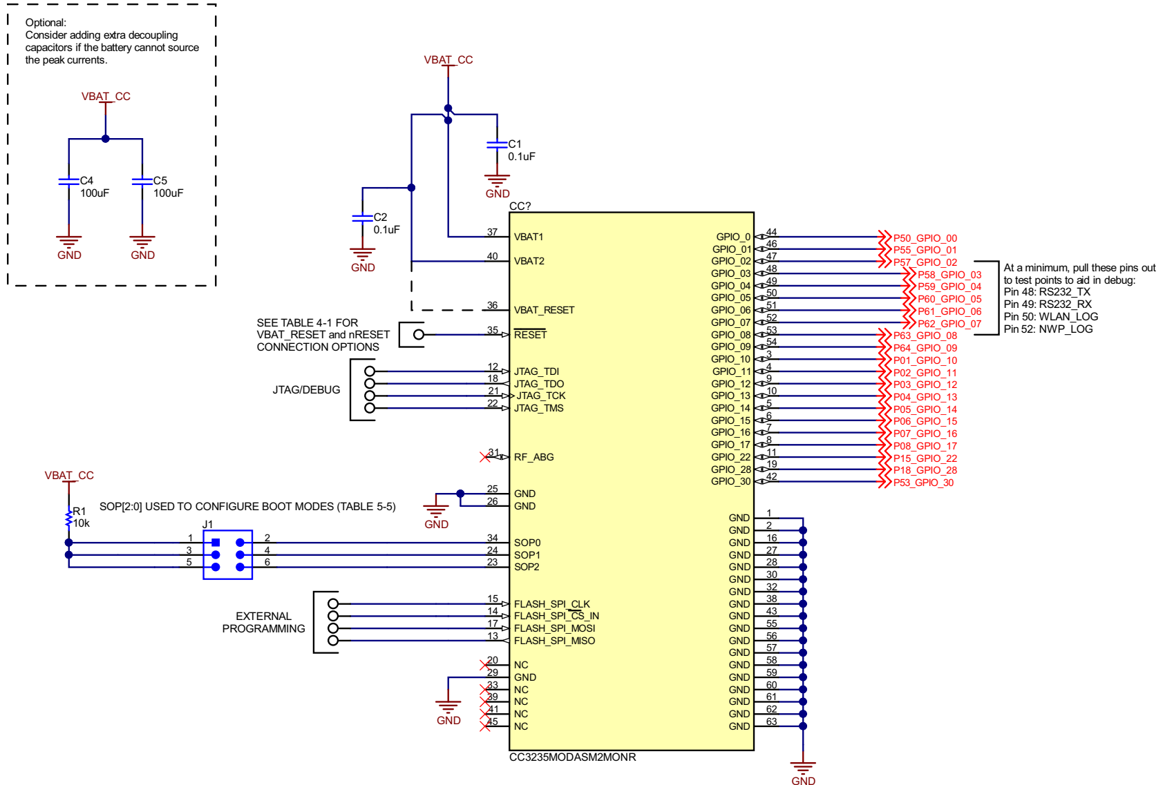
Figure 7-4. CC3235MODx Typical Application Schematic
