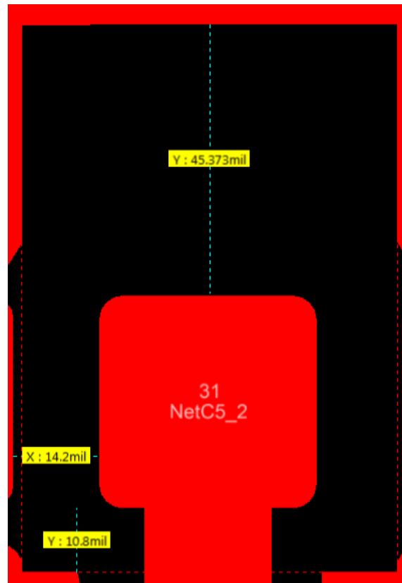
Figure 7-6. Top Layer Copper Pullback on RF Pads
