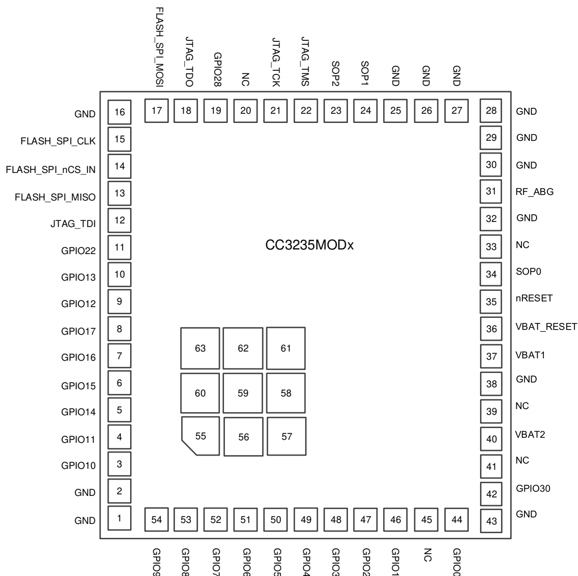
Figure 4-1. CC3235MODx Pin Diagram Bottom View
