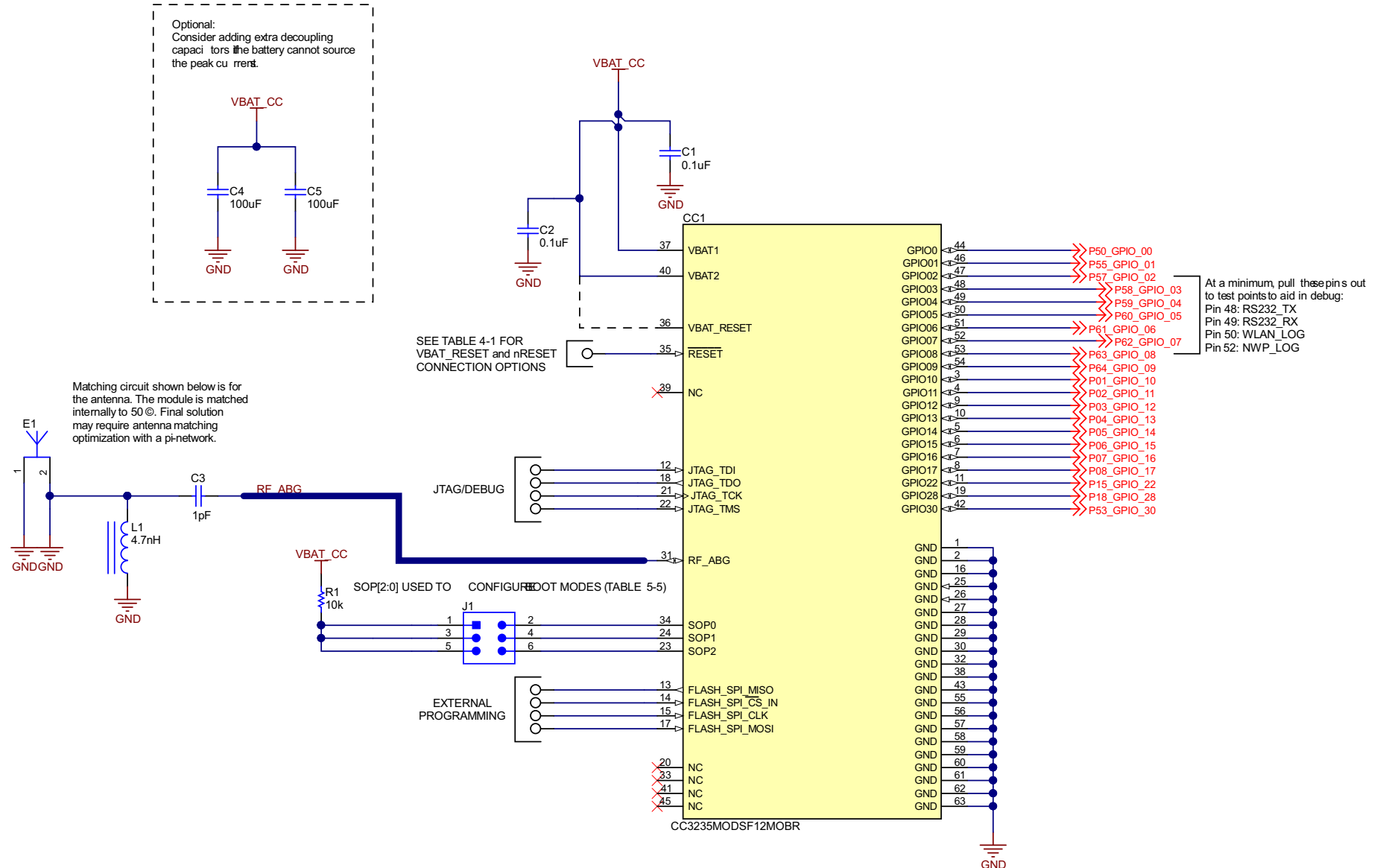
Figure 7-3. CC3235MODx Typical Application Schematic
