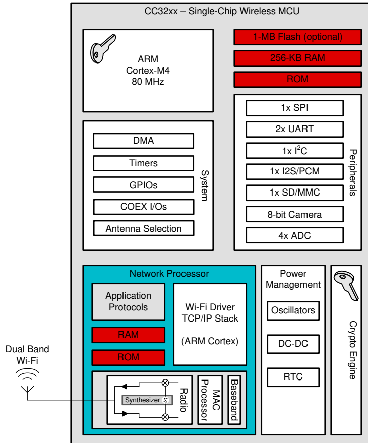
Figure 1-3. CC3235x Hardware Overview
