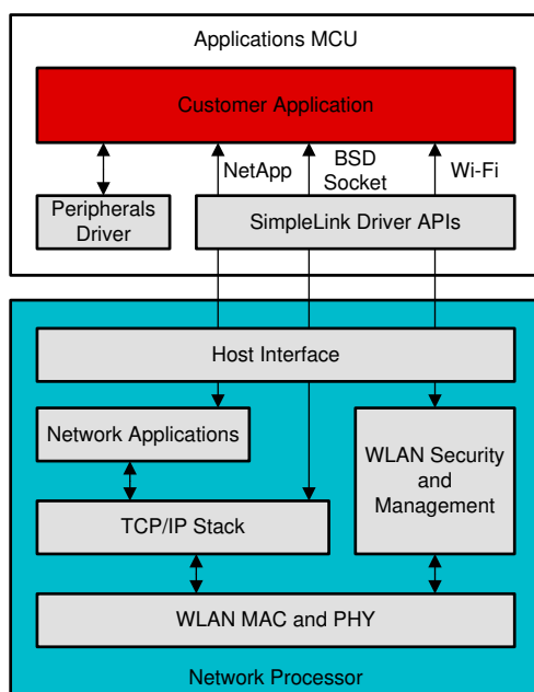
Figure 1-4. CC3235x Embedded Software Overview
