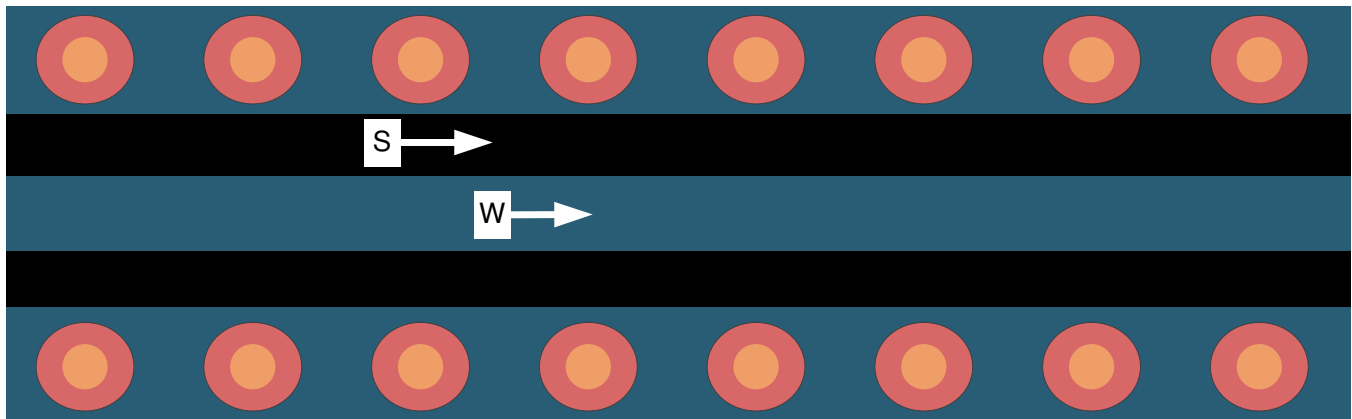
Figure 7-8. CPW With GND and Via Stitching (Top View)
