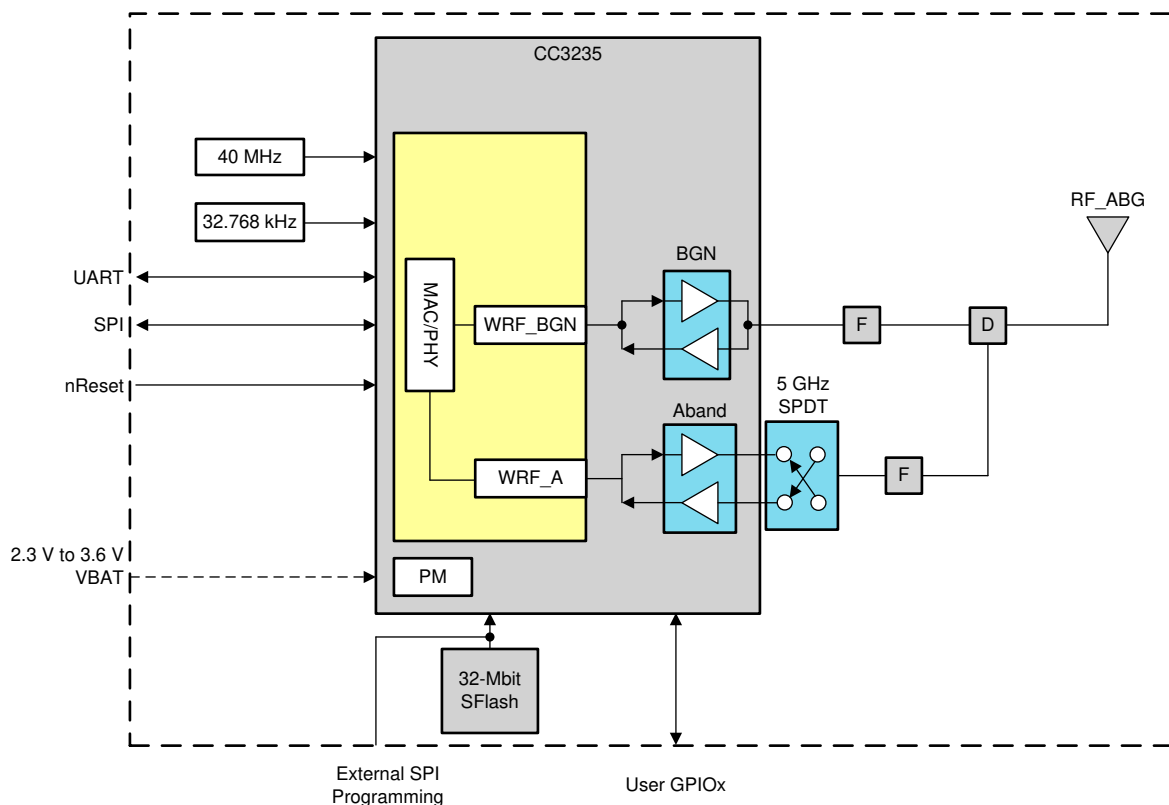
Figure 1-2. CC3235MODAx Functional Block Diagram
