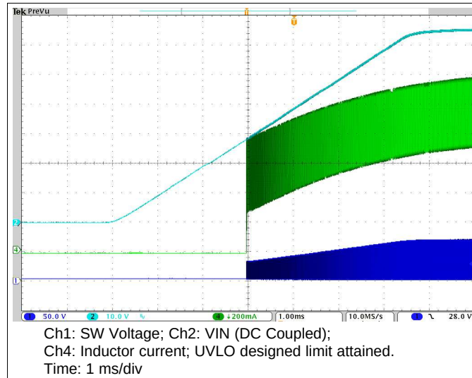
Figure 36. Startup Transient
