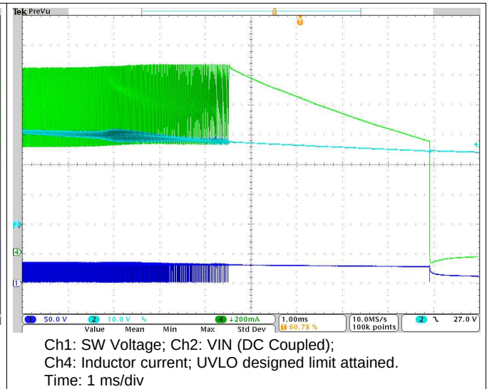
Figure 37. Shut-Down Transient
