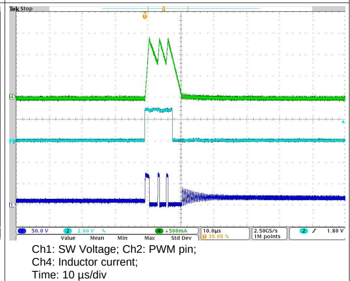
Figure 39. PWM Dimming: 250Hz, 0.25% Duty Cycle
