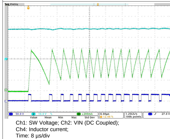
Figure 38. First 15 SW Node Pulses at Turn-On
