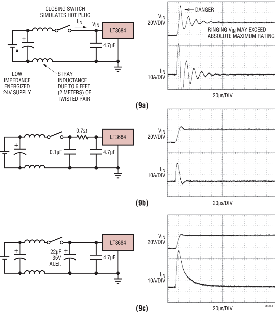
Figure 9. A Well Chosen Input Network Prevents Input Voltage Overshoot and Ensures Reliable Operation when the LT3684 Is Connected to a Live Supply
