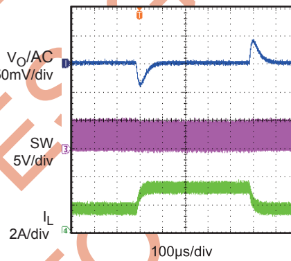
Load Transient I_O = 1.5A to 3A
