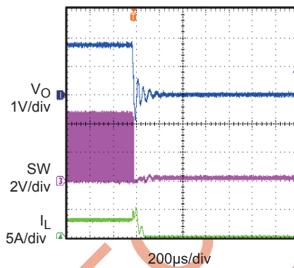
Short Circuit Protection I_O = 3A to short
