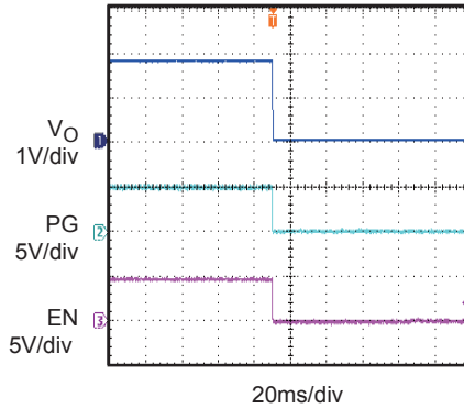
Shut-down through EN I_O = 3A
