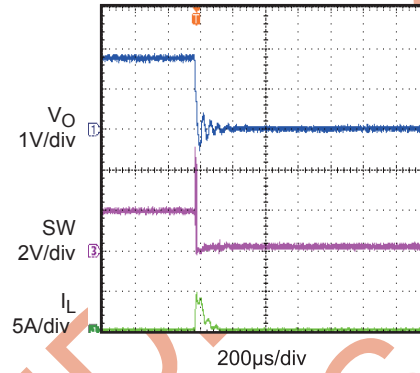
Short Circuit Protection I_O = 0A to short
