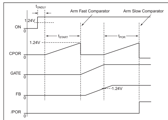
FIGURE 1-3: Power-On Start-Up Delay Timing.
