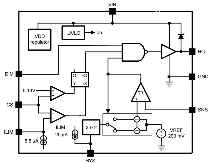
Figure 14. Block Diagram
