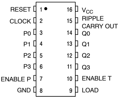
Figure 1. Pin Assignment
