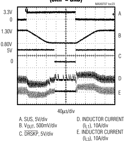
SUSPEND TRANSITION (SKIP = GND)
