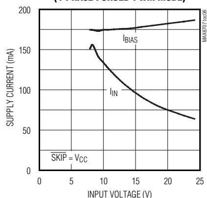
NO-LOAD SUPPLY CURRENT vs. INPUT VOLTAGE (4-PHASE FORCED-PWM MODE)
