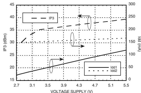
Output IP3 and Idd vs. Supply Voltage @ 2200 MHz [3]
