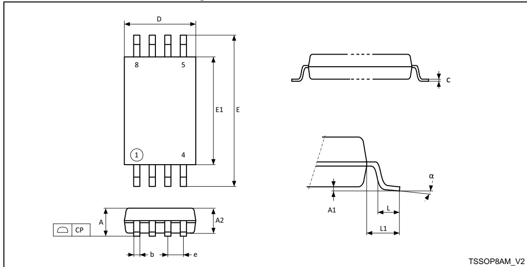
Figure 27. TSSOP8 outline
