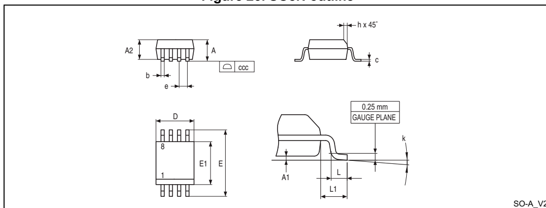
Figure 23. SO8N outline
