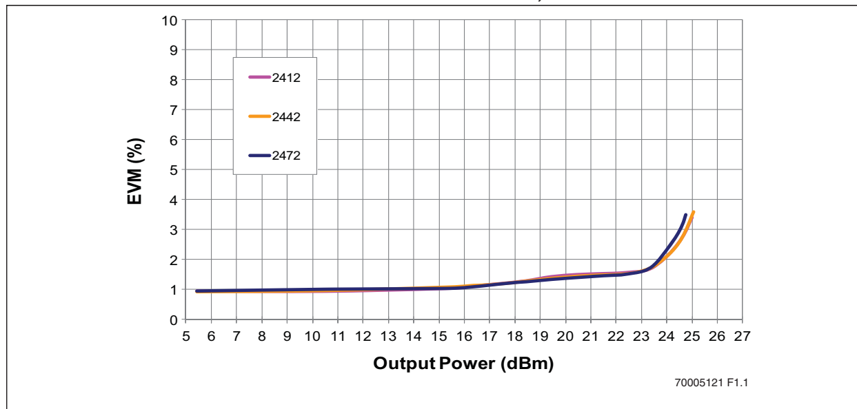
FIGURE 6-2: DYNAMIC EVM VERSUS OUTPUT POWER, 23% DUTY CYCLE
