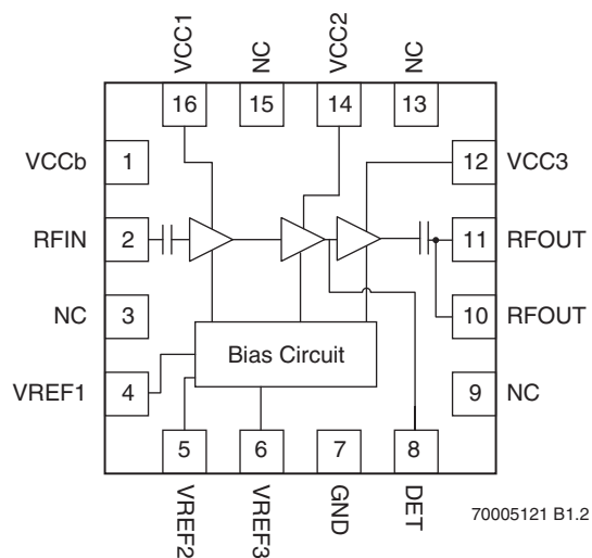
FIGURE 1-1: FUNCTIONAL BLOCK DIAGRAM
