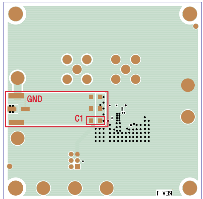
Figure 3. Bottom Layer of DC2593A
