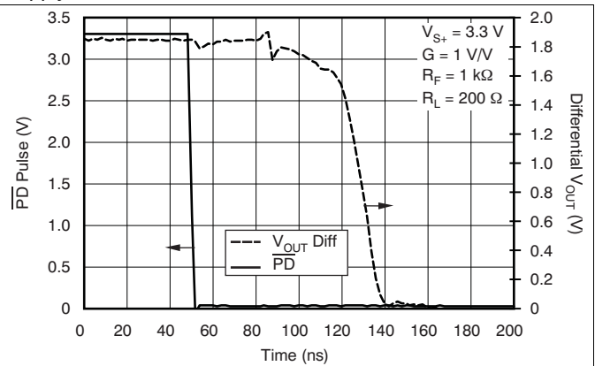
Figure 20. Turn-Off Time
