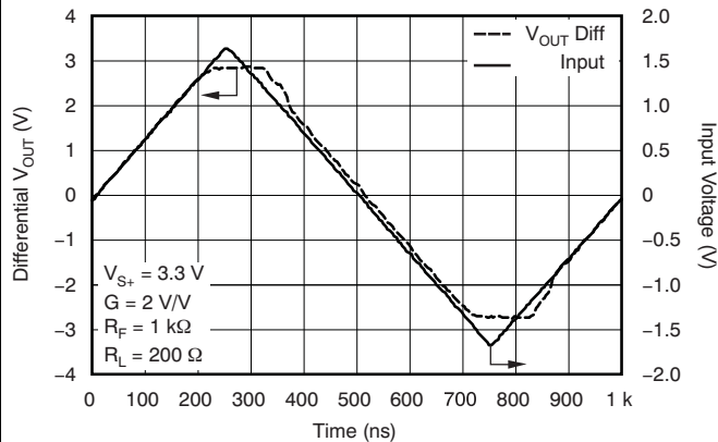
Figure 5. Overdrive Recovery
