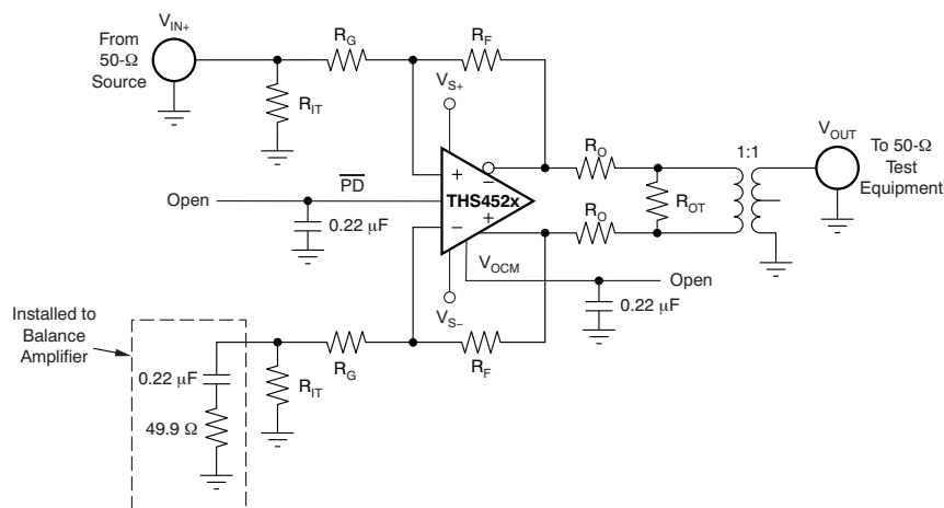
Figure 55. Distortion Test Circuit
