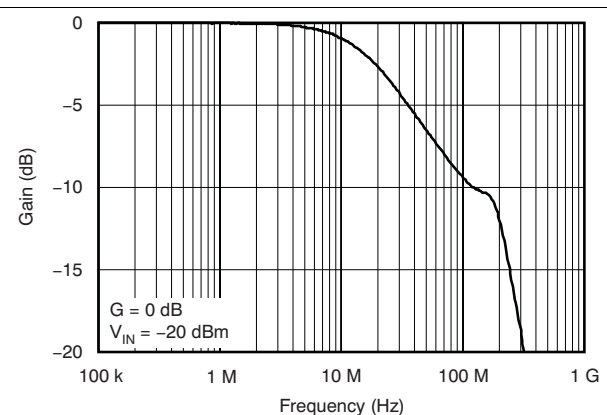
Figure 24. V_{OCM} Small-Signal Frequency Response
