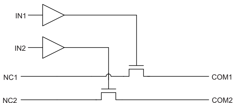
Simplified Schematic
