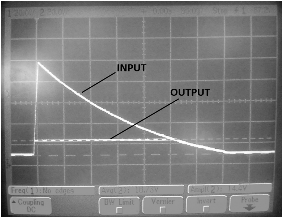
Figure 3: ISO-7637-2 Load Dump Event
