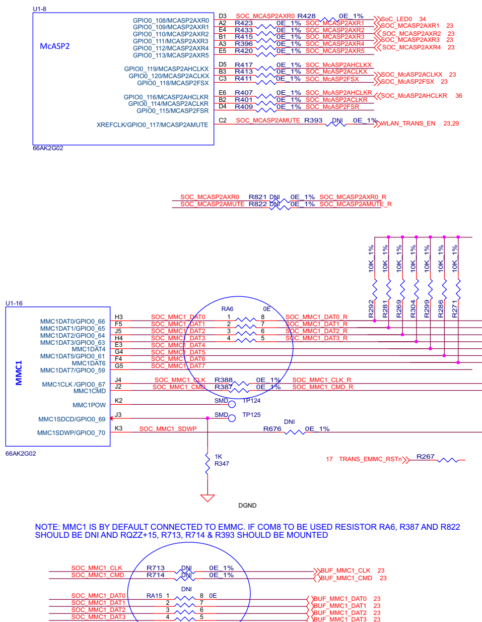
Figure 18. eMMC and COM8 Resistor Multiplexing
