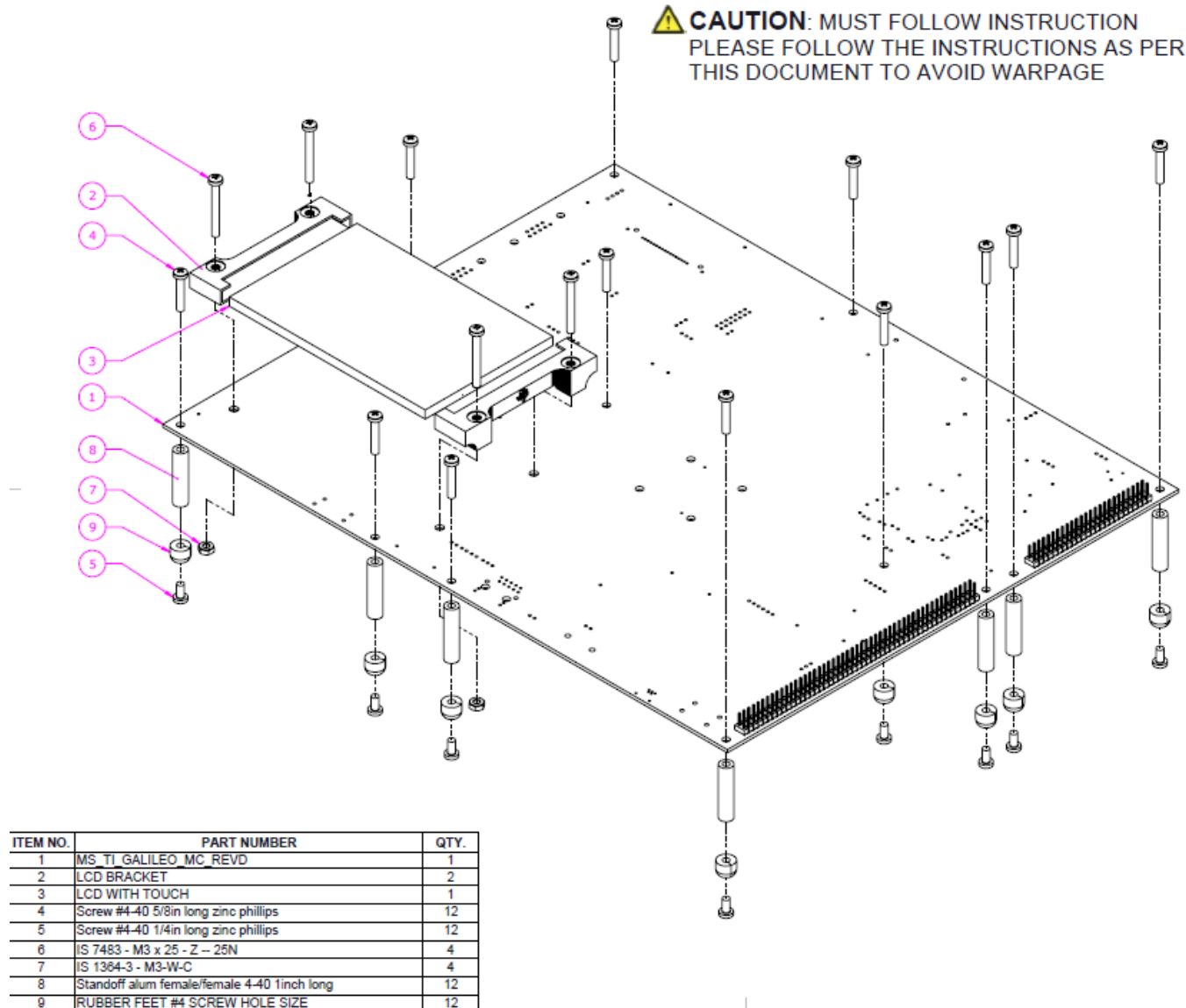
Figure 41. EVMK2G Mechanical Drawing
