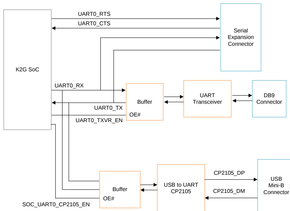
Figure 29. UART0 Interface Block Diagram
