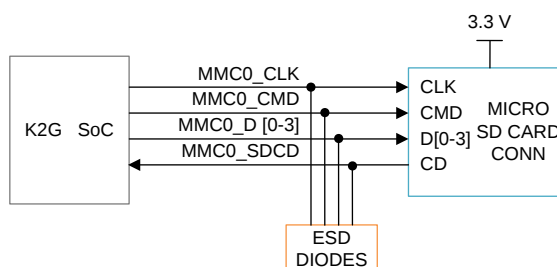
Figure 16. SD/MMC Interface Block Diagram
