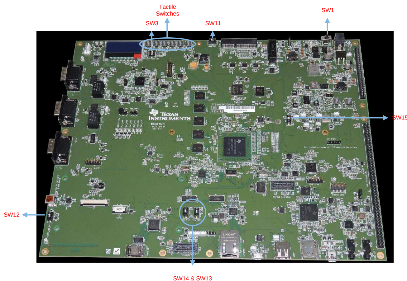
Figure 39. EVMK2G Switches
