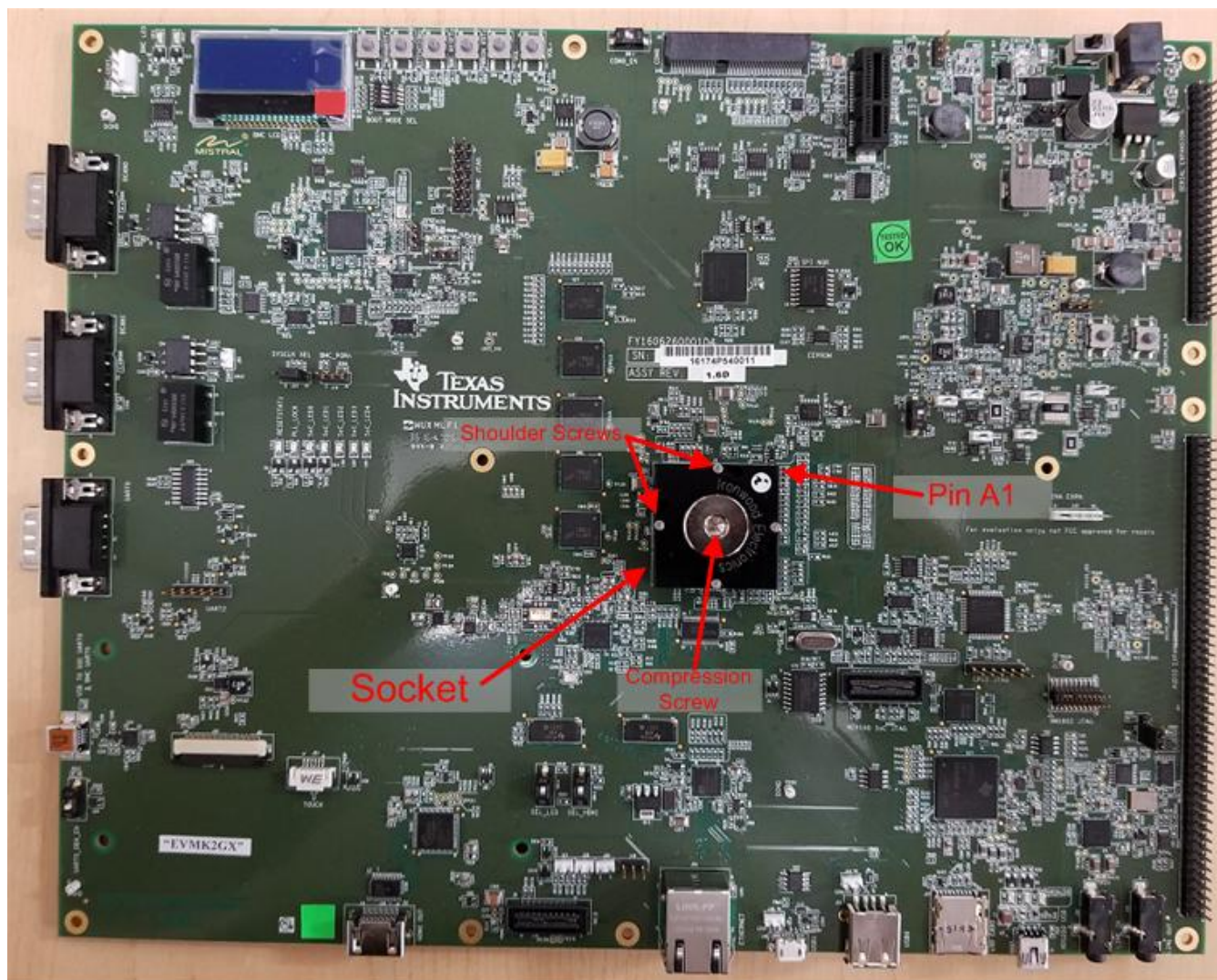
Figure 48. Ironwood Socket
