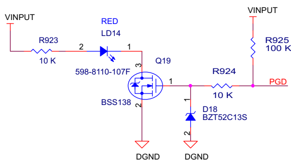
Figure 5. Fault Indication Circuit
