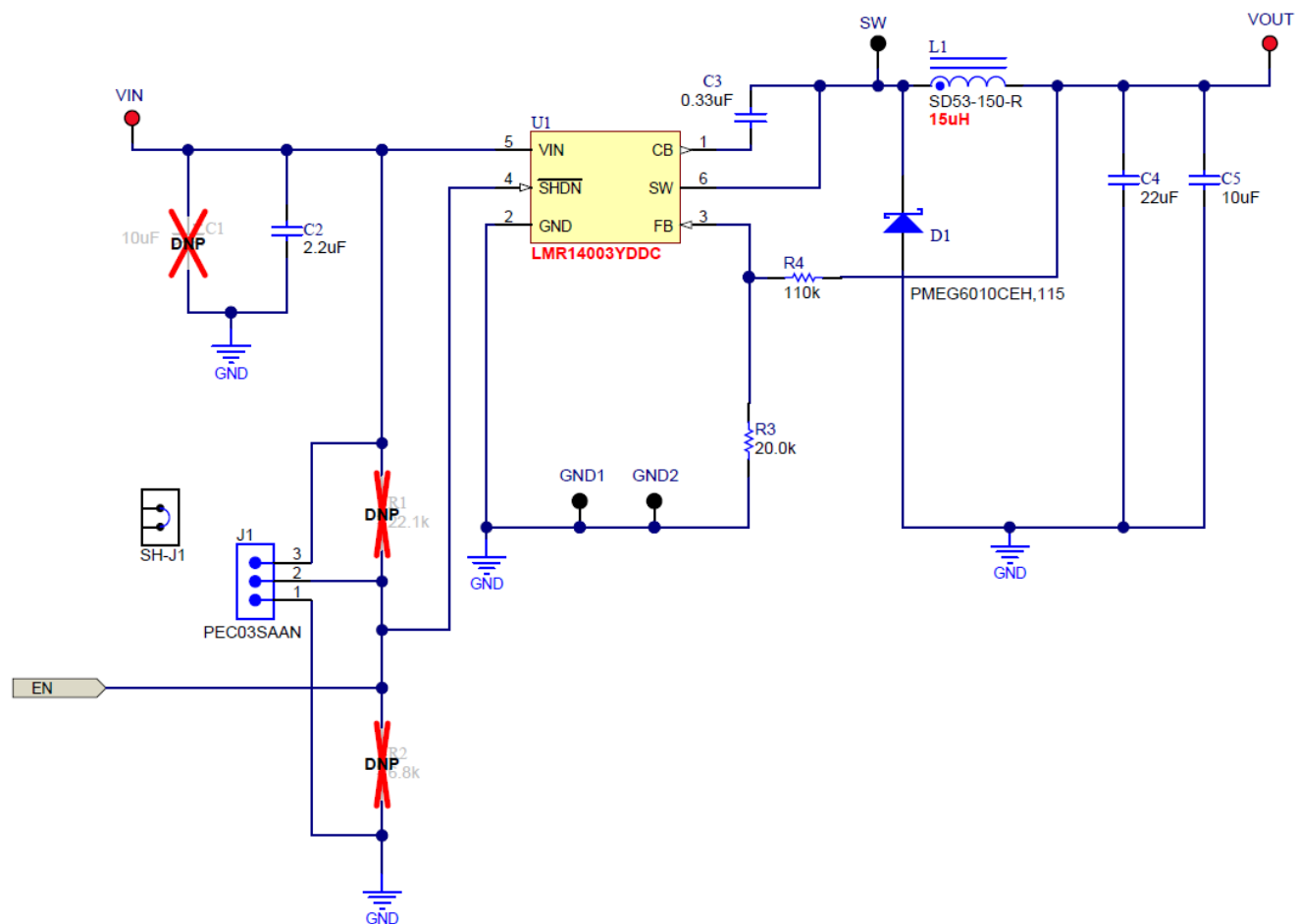
Figure 5. LMR14006YEVM Schematic
