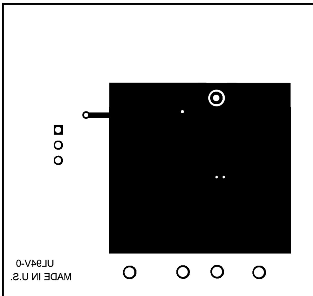
Figure 4. Bottom Layer
