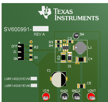
Figure 1. LMR14003Y/6YEVM Board
