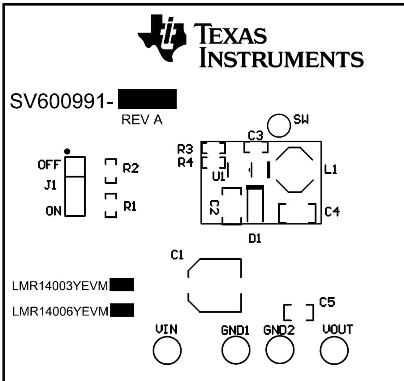
Figure 3. Top Layer
