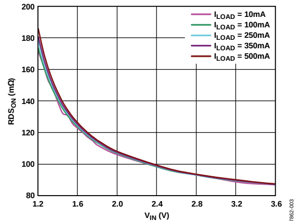
Figure 3. R_{DS_{ON}} vs. Input Voltage, V_{IN} (Includes ~15 mΩ Trace Resistance)
