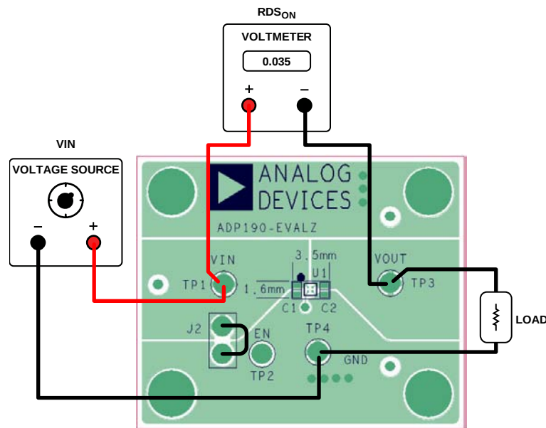
Figure 4. R_{DS_{ON}} Measurement
