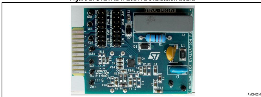
Figure 2: STEVAL-IPE014V1 evaluation board
