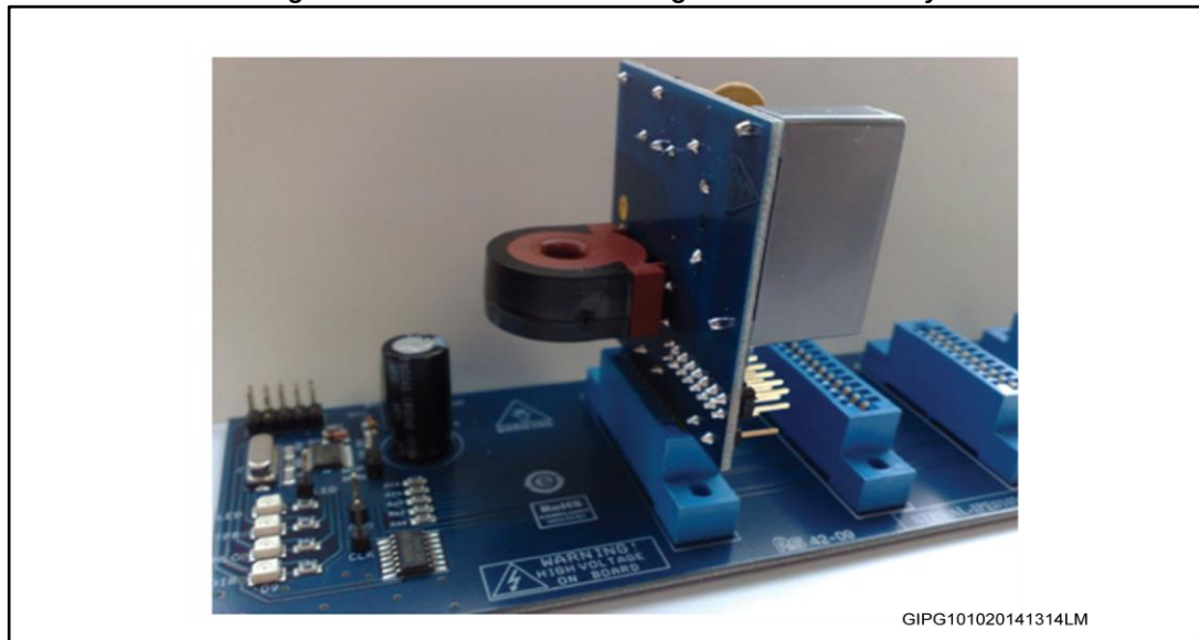
Figure 3: STEVAL-IPE010V2 daughterboard assembly
