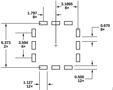
7.2mm × 7.2mm STACKED LGA. ALL DIMENSIONS IN mm.
