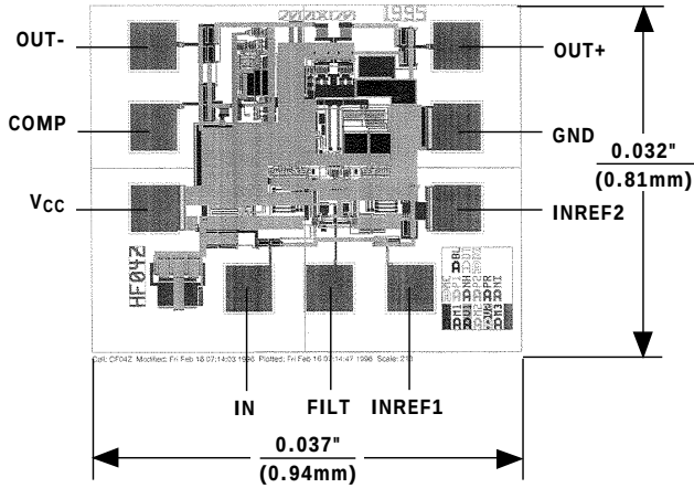
Chip Topography
